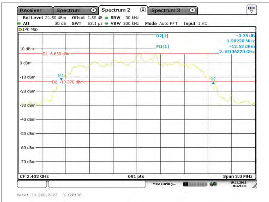
2DH5_Ant1_2402
