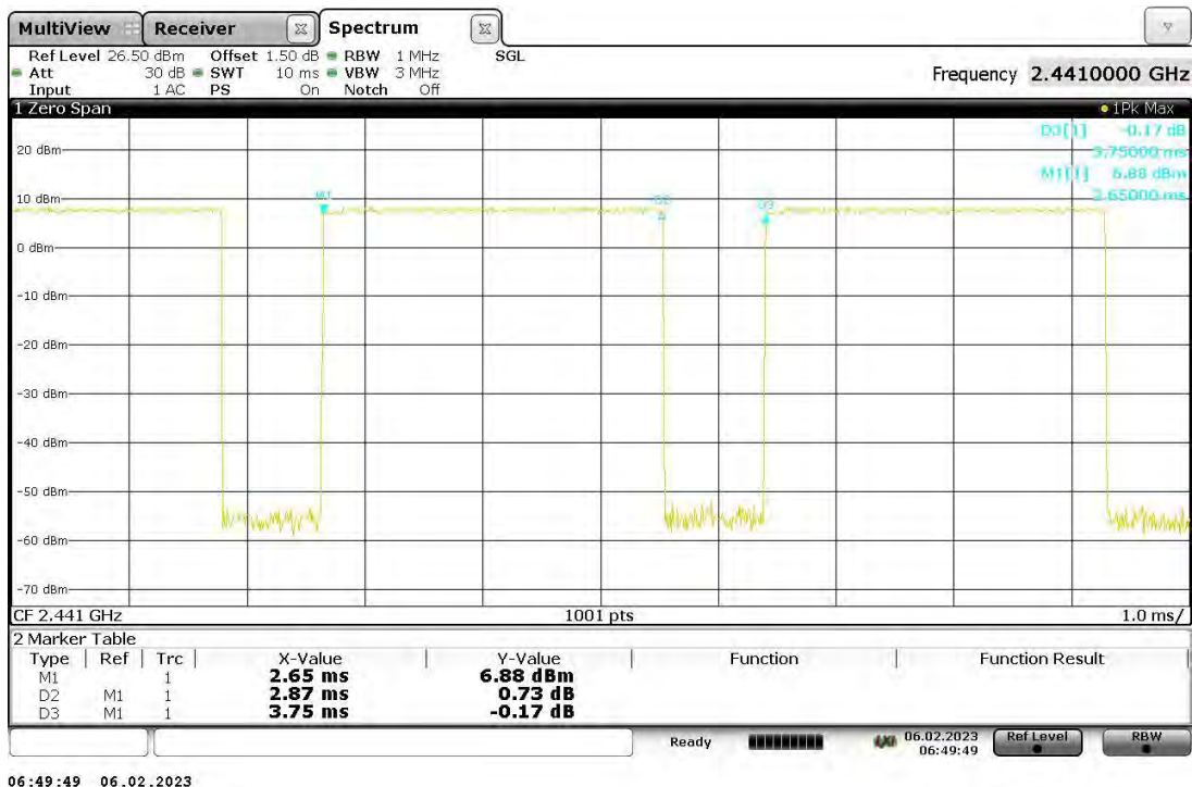
2DH5_Ant1_2441
