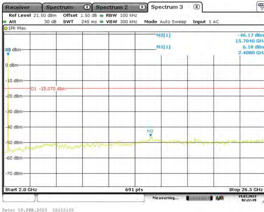
3DH5_Ant1_2402_2000~26500
