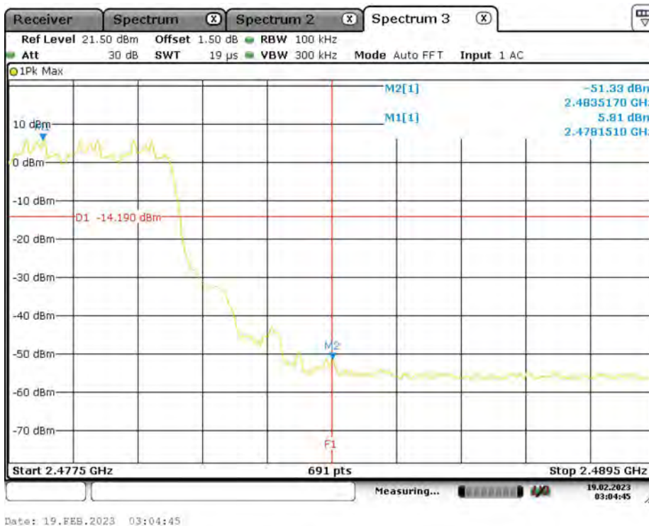
3DH5_Ant1_High_Hop_2480
