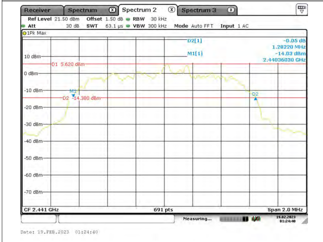
2DH5_Ant1_2441
