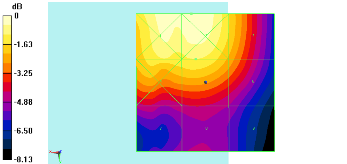
Fig B.3 HAC RF E-Field LTE Band41 PC2 QPSK CH41055
