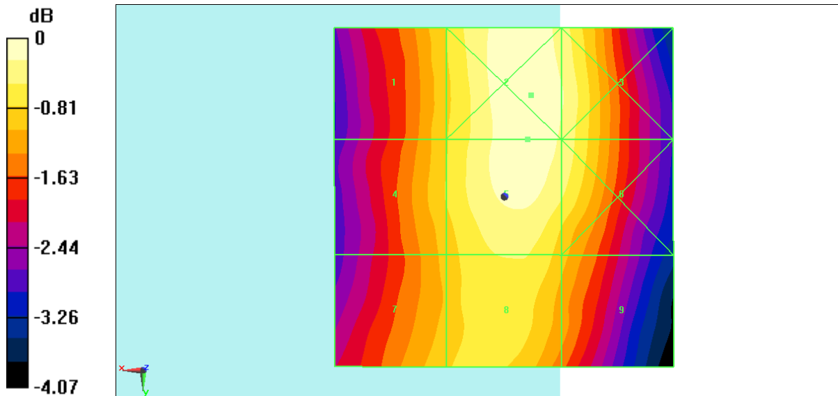
Fig B.1 HAC RF E-Field GSM 850 Middle
