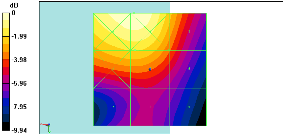
Fig B.2 HAC RF E-Field LTE Band41 QPSK PC2
