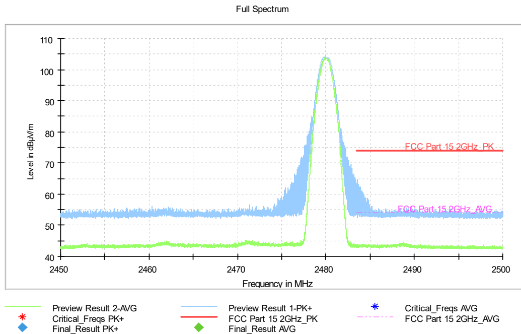
Fig.14. Frequency Band Edges: GFSK, Channel 78, Hopping Off, 2.45 GHz - 2.50GHz
