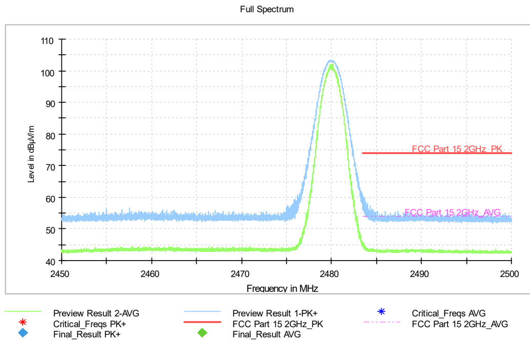
Fig.18. Frequency Band Edges: 8DPSK, Channel 78, Hopping Off, 2.45 GHz - 2.50GHz
