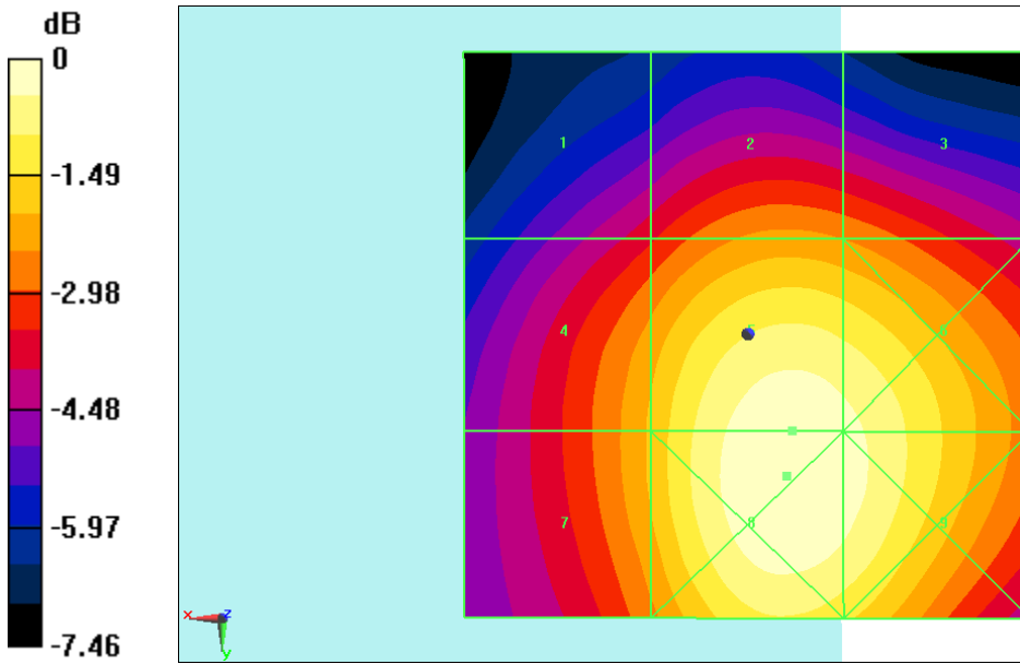
Fig B.5 HAC RF E-Field WIFI2.4G
