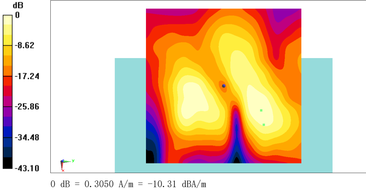
Fig B.3 T-Coil LTEB41
