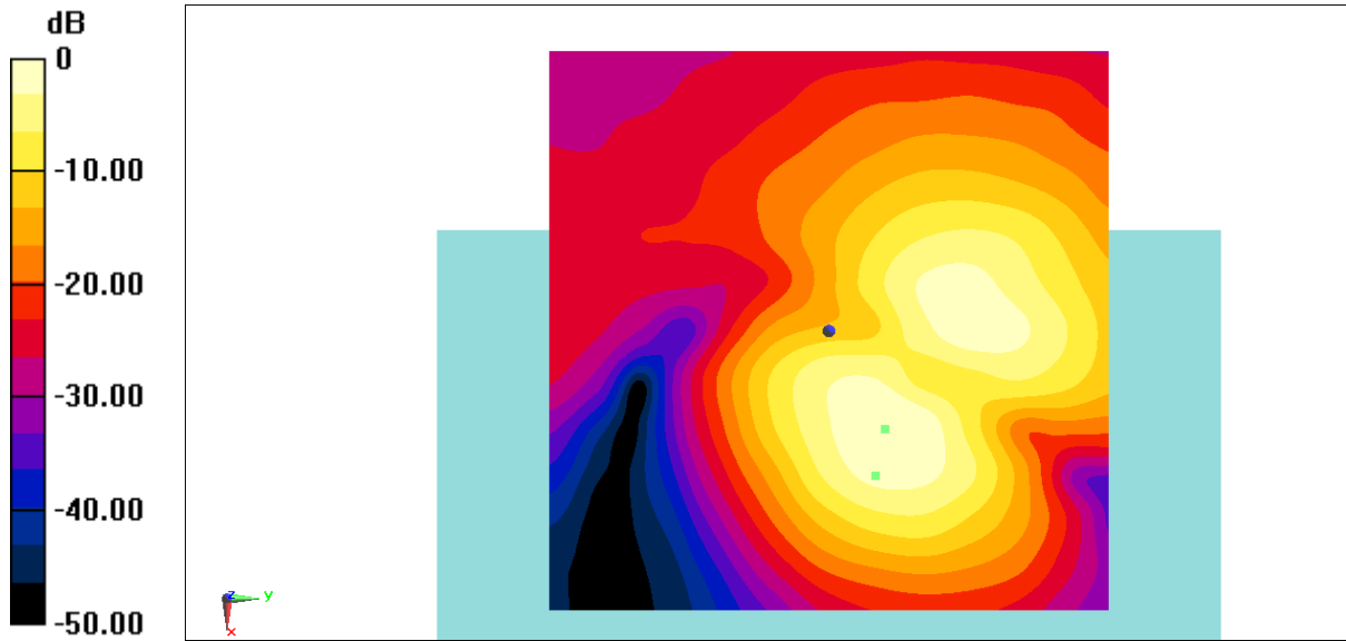
Fig B.4 T-Coil LTE Band 41
