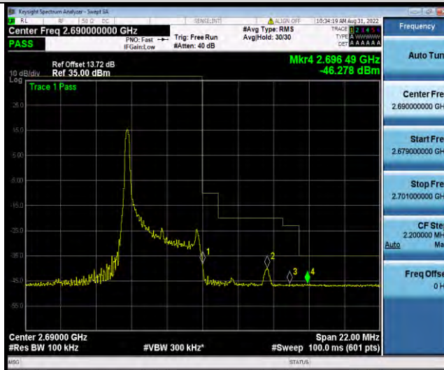
Band41-5MHz-QPSK-41565-1RB#24
