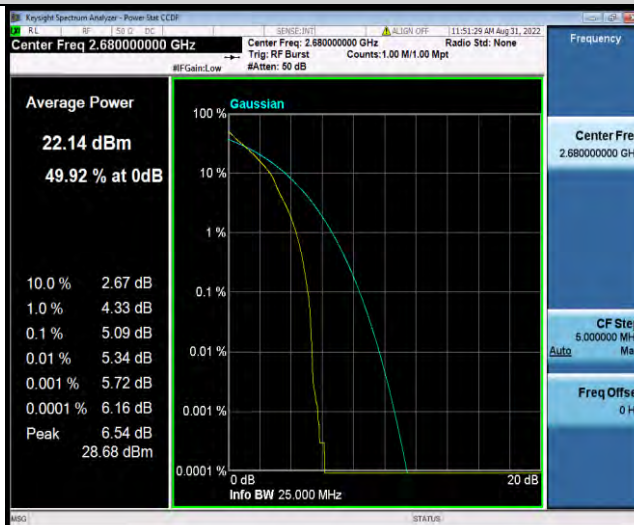
Band41-20MHz-QPSK-41490-100RB#0
