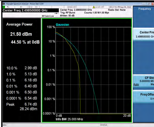
Band41-5MHz-64QAM-39675-25RB#0
