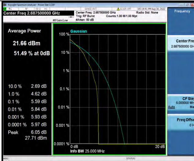
Band41-5MHz-QPSK-41565-25RB#0
