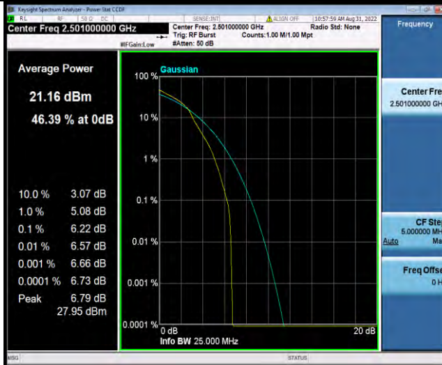
Band41-10MHz-16QAM-39700-50RB#0
