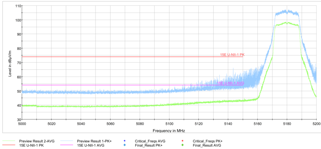
Fig.34 Band Edges (802.11a Ch36, 5180MHz)
