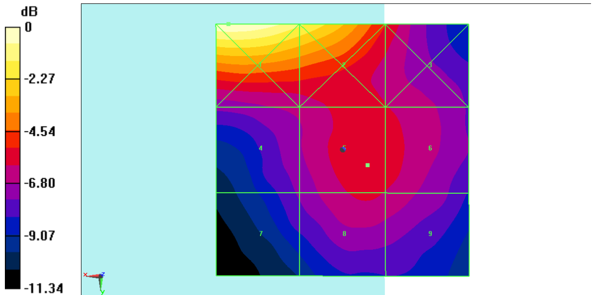
Fig B.1 HAC RF E-Field LTE Band43 QPSK
