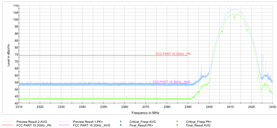
Fig.A.6.2.1 Transmitter Spurious Emission - Radiated (Power): 802.11b, ch1, 2.31 GHz – 2.43GHz
