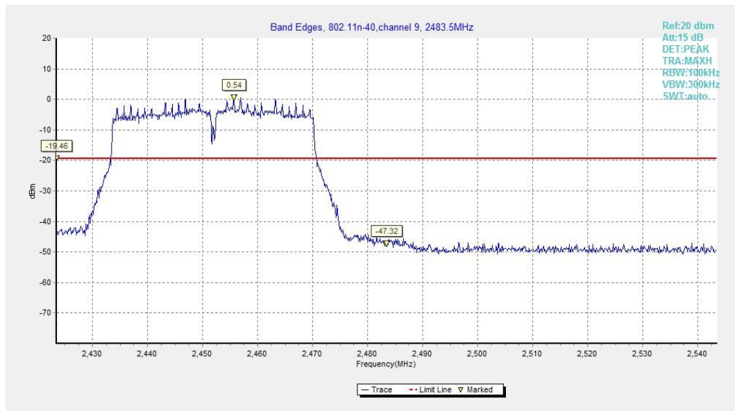
Fig.A.5.8 Band Edges (802.11n-HT40, Ch 9)
