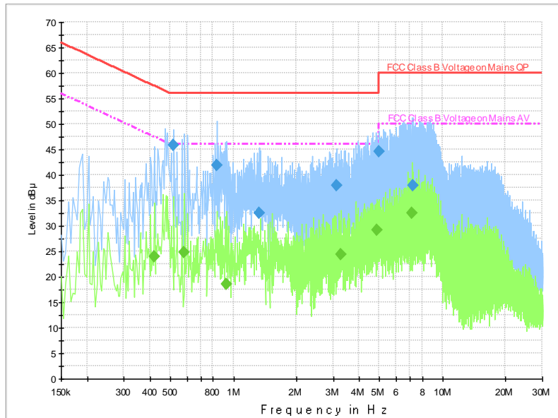
Fig.B.9.1 AC Powerline Conducted Emission- bluetooth
