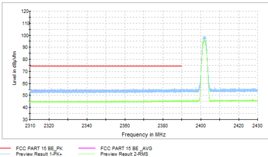
Fig.3. Frequency Band Edges: GFSK, 2402 MHz, Hopping Off, 2.31 GHz – 2.43GHz
