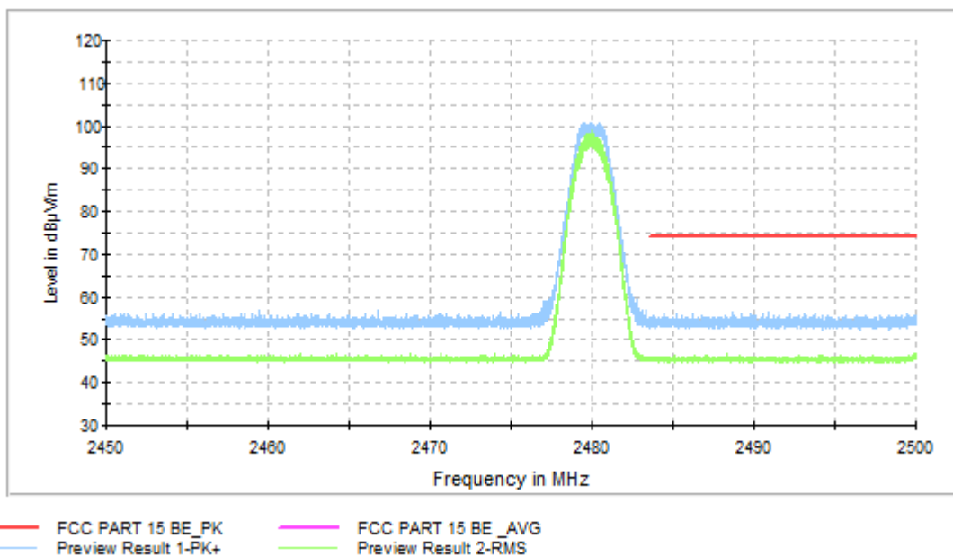
Fig.4. Frequency Band Edges: GFSK, 2480 MHz, Hopping Off , 2.45 GHz - 2.50GHz
