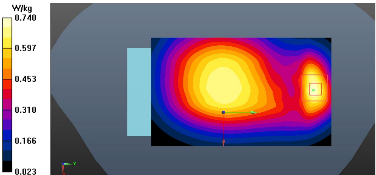
Fig.2 GSM850 Body
