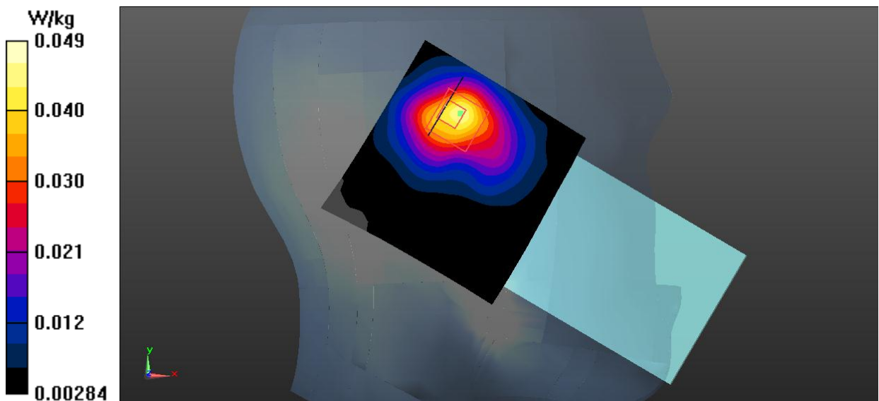
Fig.23 Bluetooth Head
