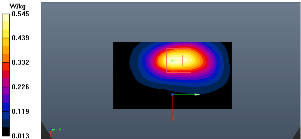
Fig.4 GSM1900 Body
