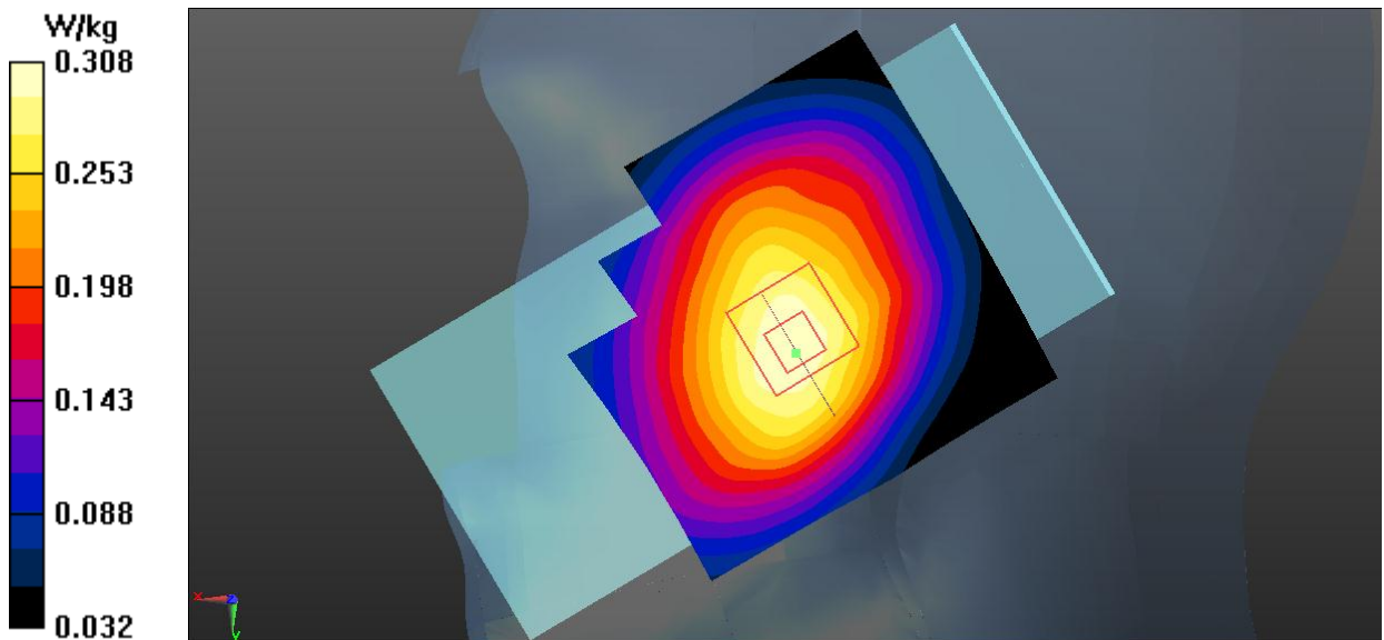
Fig.1 GSM850 Head
