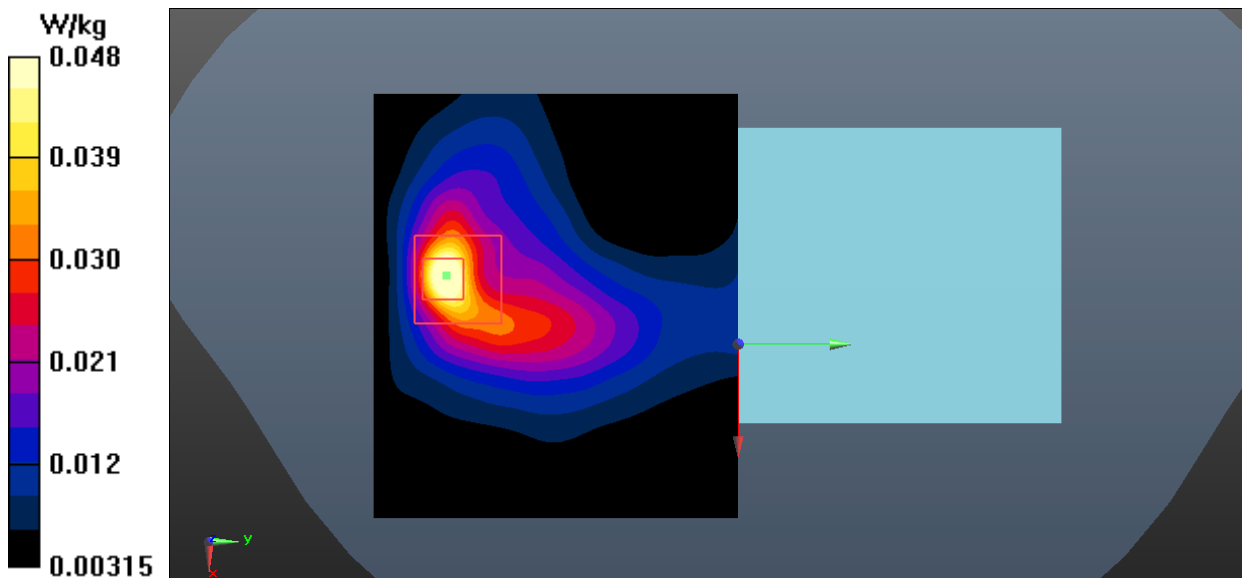
Fig.24 Bluetooth Body
