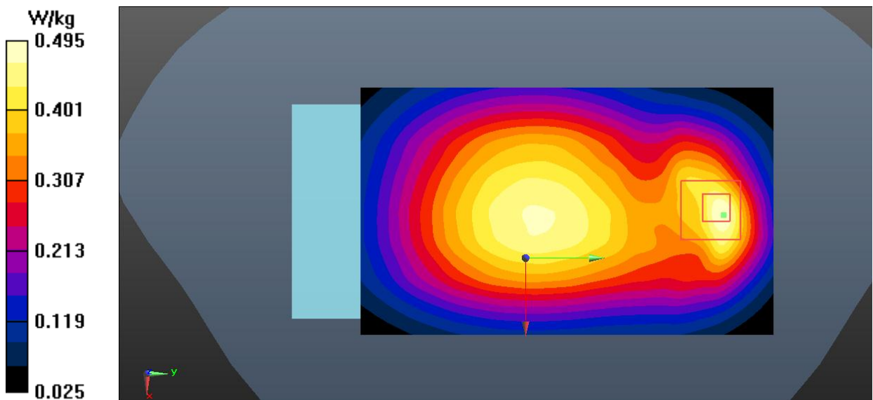
Fig.20 LTE Band 13 Body
