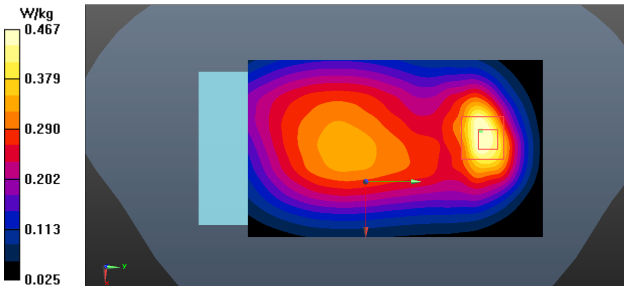
Fig.14 LTE Band 5 Body
