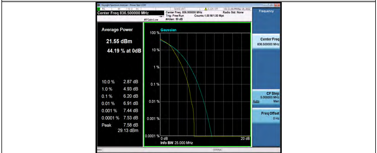
Band5-3MHz-16QAM-20635-1RB#0
