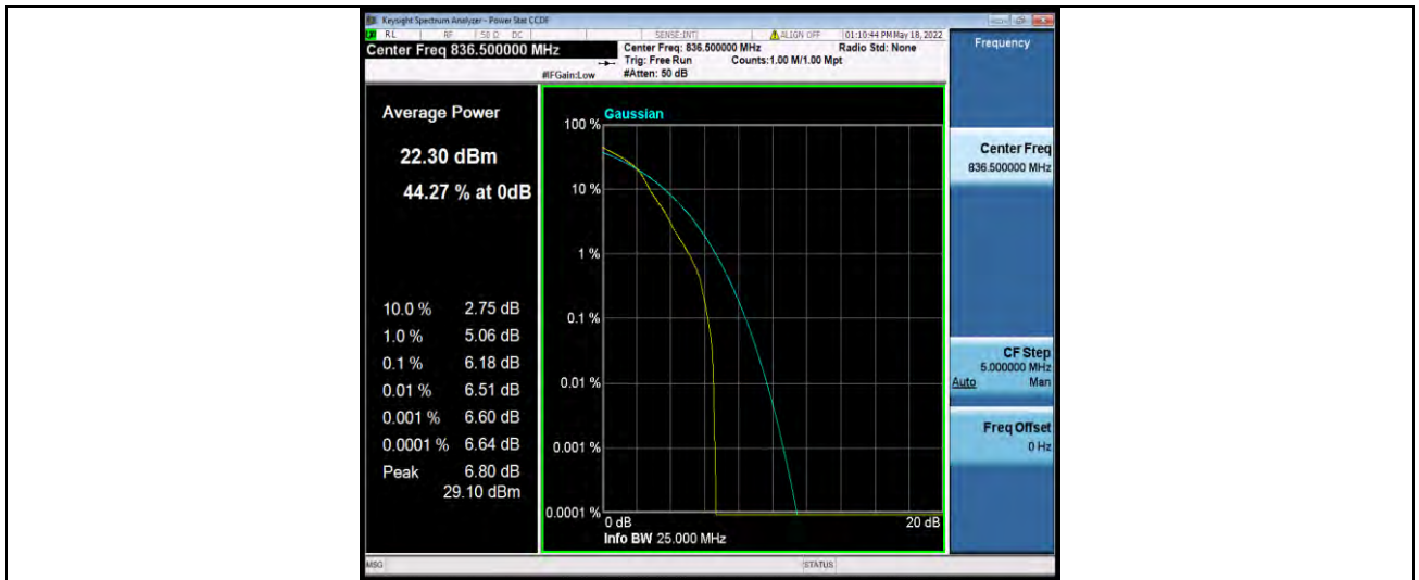
Band5-3MHz-16QAM-20525-15RB#0
