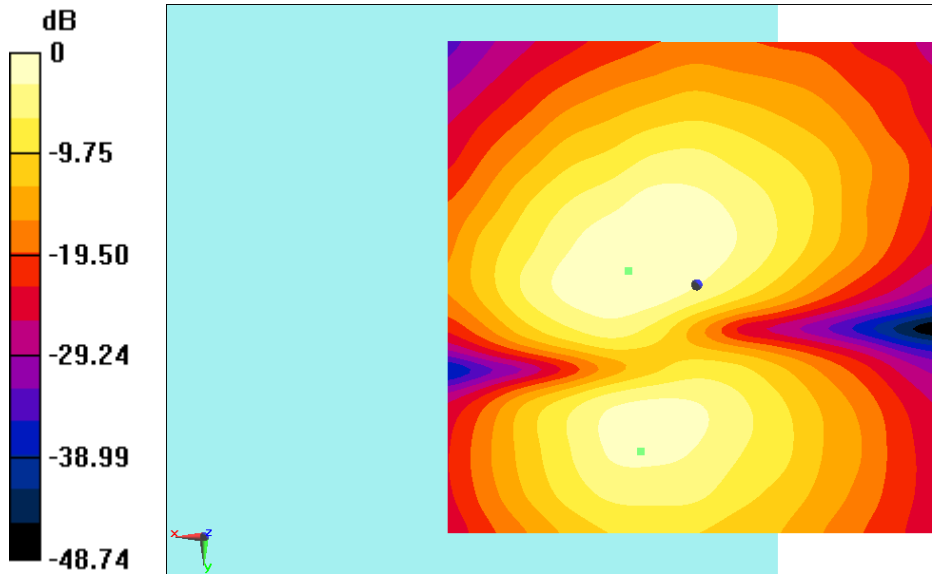
Fig B.1 T-Coil GSM 850
