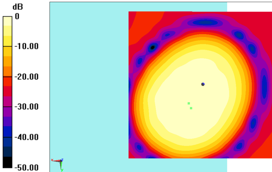
Fig B.2 T-Coil LTE Band 2
