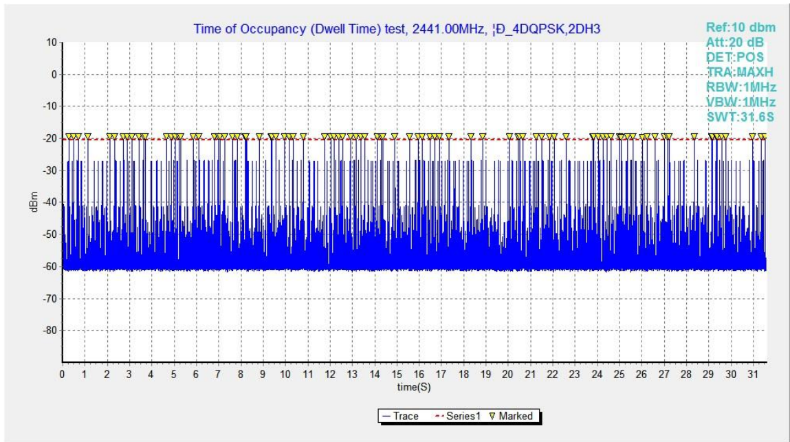
Fig.52. Number of Transmissions Measurement: Channel 39,Packet 2-DH3
