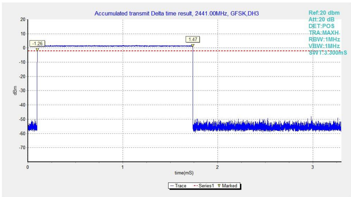
Fig.45. Time of occupancy (Dwell Time): Channel 39, Packet DH3
