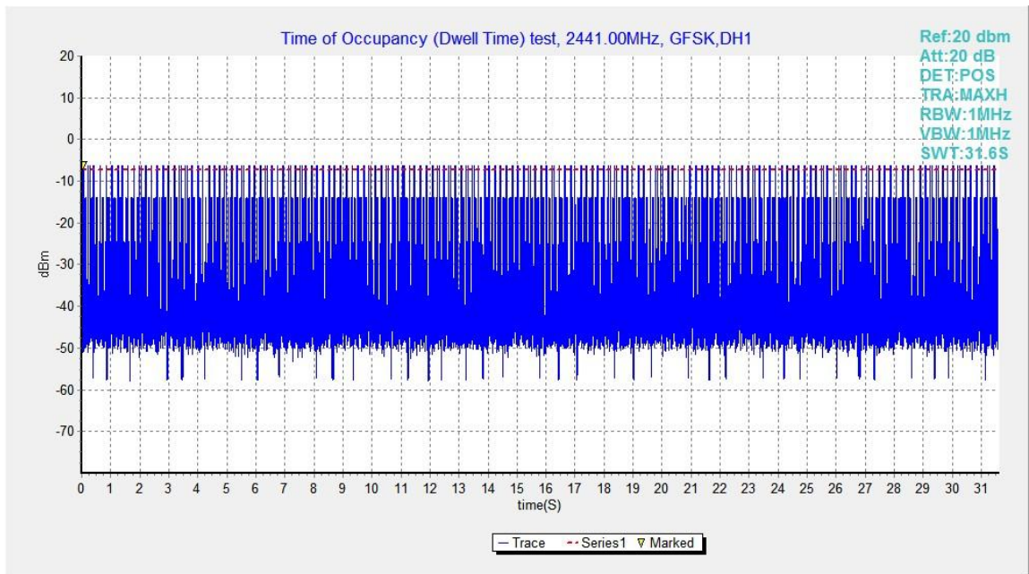
Fig.44. Number of Transmissions Measurement: Channel 39,Packet DH1
