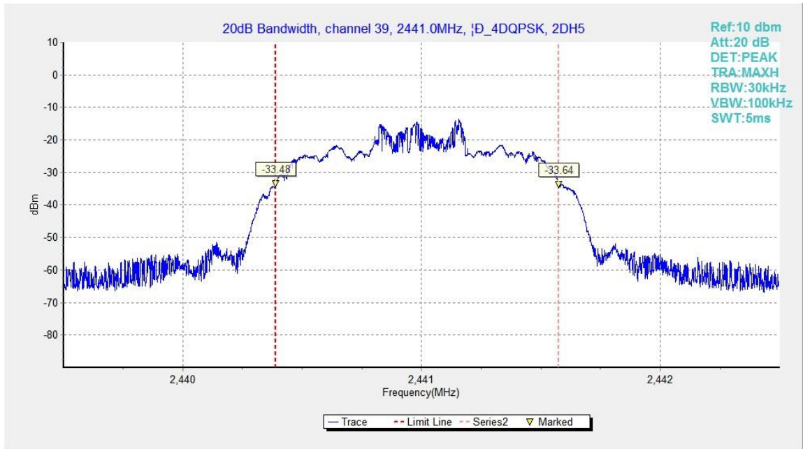
Fig.59. 20dB Bandwidth: \pi/4 DQPSK, Channel 39
