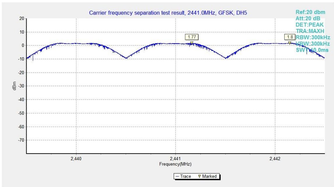
Fig.61. Carrier frequency separation measurement: GFSK, Channel 39
