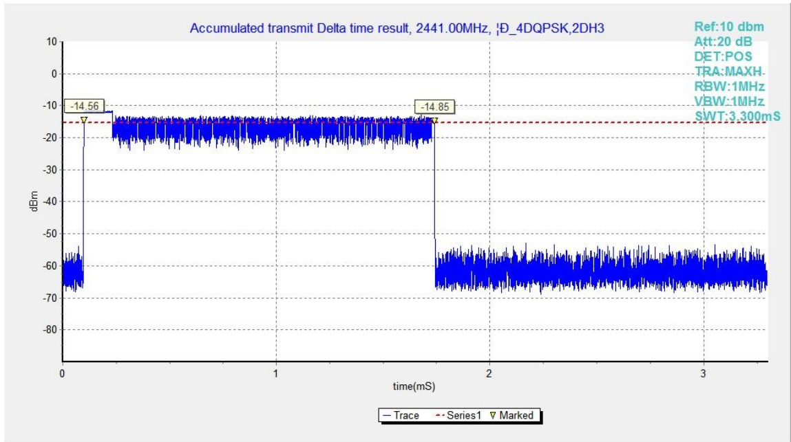
Fig.51. Time of occupancy (Dwell Time): Channel 39, Packet 2-DH3
