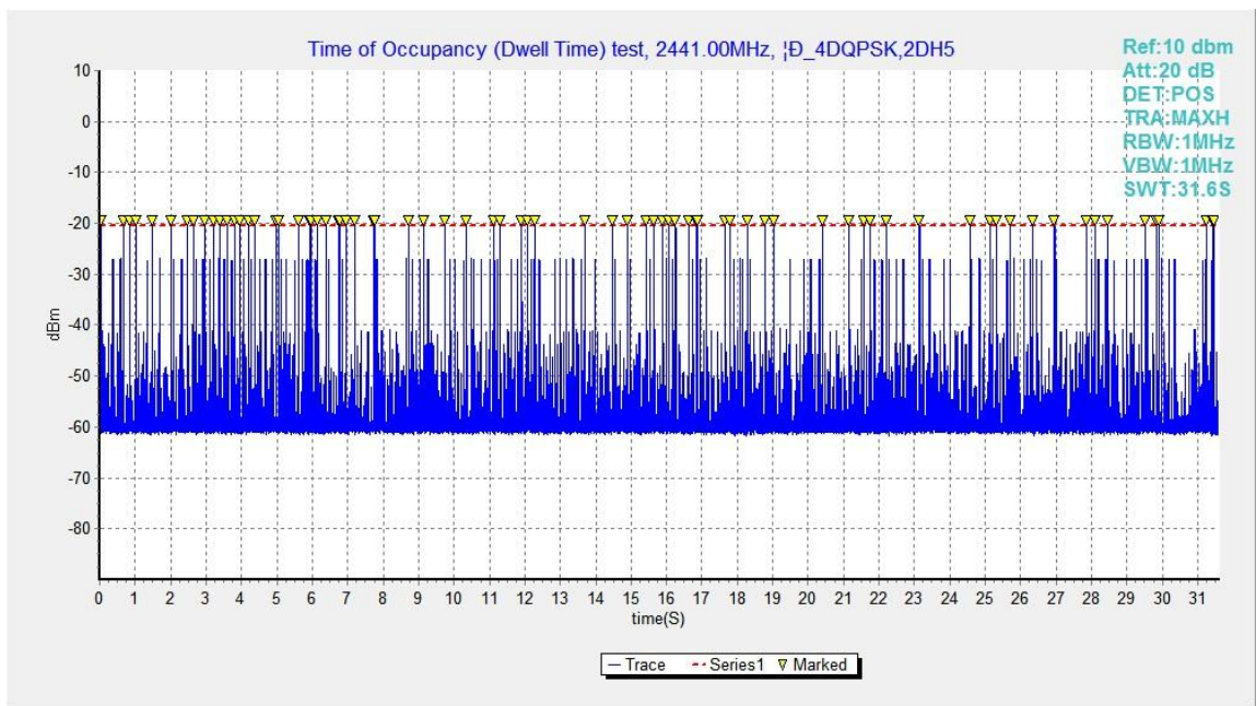
Fig.54. Number of Transmissions Measurement: Channel 39,Packet 2-DH5
