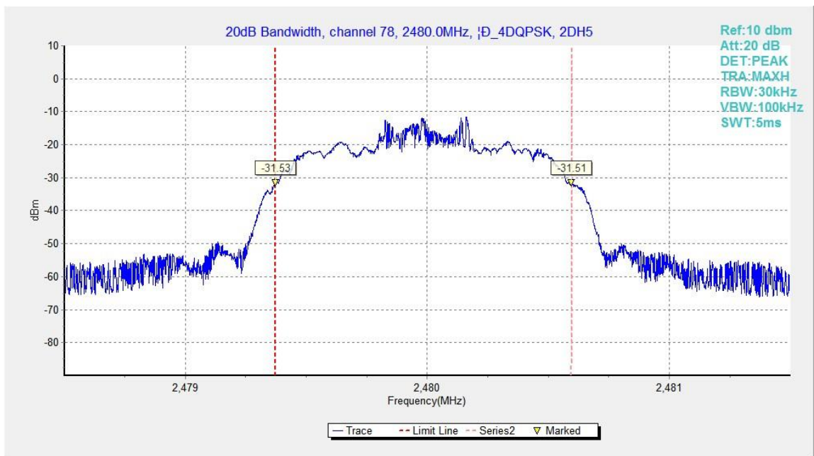
Fig.60. 20dB Bandwidth: \pi/4 DQPSK, Channel 78
