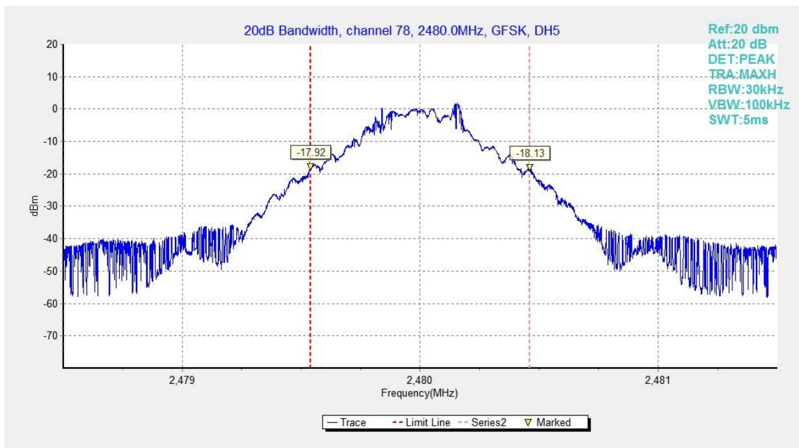
Fig.57. 20dB Bandwidth: GFSK, Channel 78
