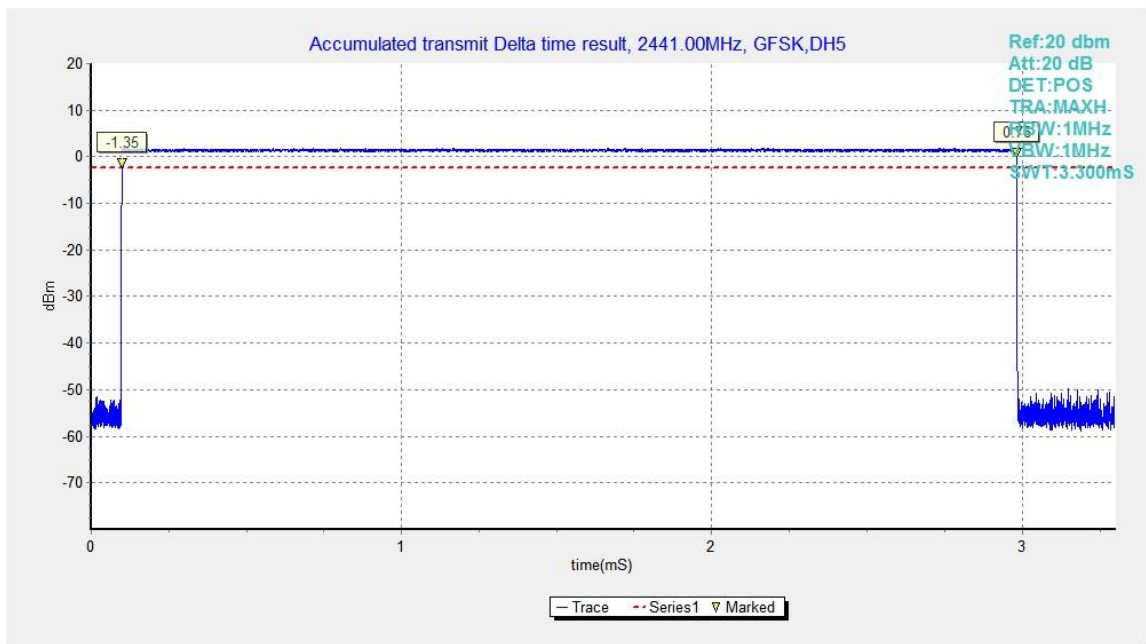
Fig.47. Time of occupancy (Dwell Time): Channel 39, Packet DH5
