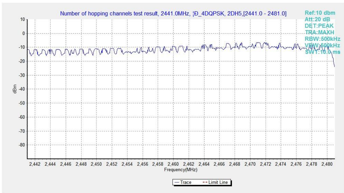
Fig.66. Number of hopping frequencies: \pi/4 DQPSK, Channel 40 - 78
