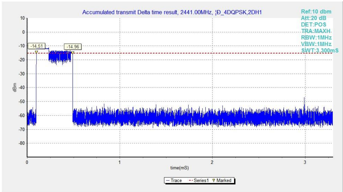
Fig.49. Time of occupancy (Dwell Time): Channel 39, Packet 2-DH1
