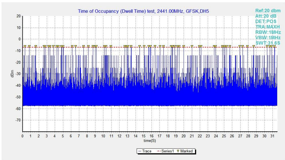
Fig.48. Number of Transmissions Measurement: Channel 39,Packet DH5
