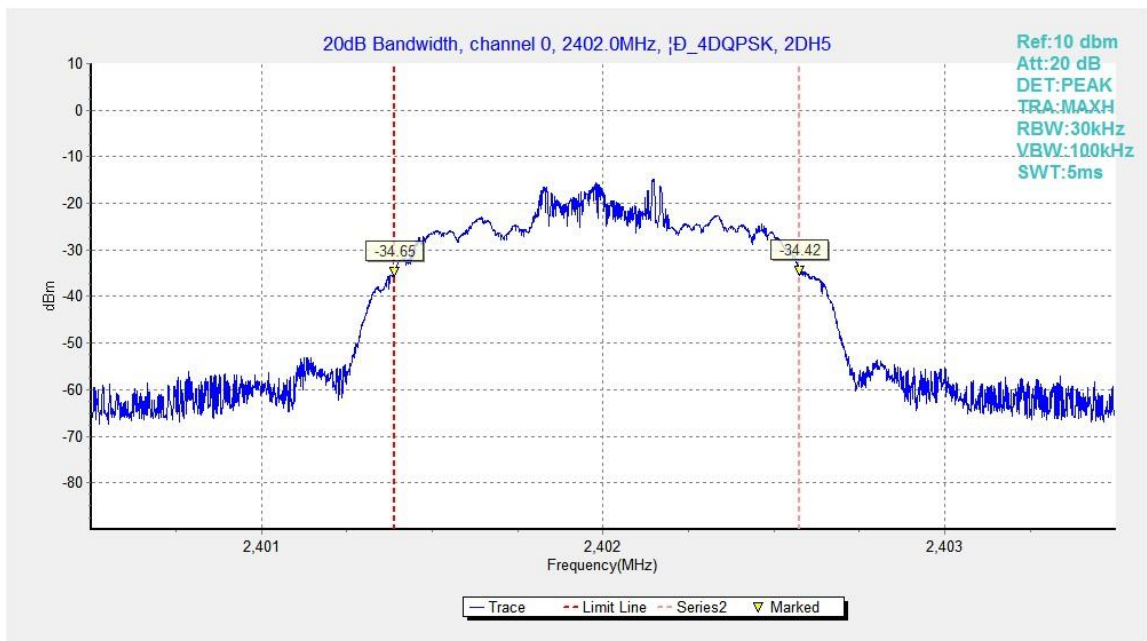
Fig.58. 20dB Bandwidth: \pi/4 DQPSK, Channel 0
