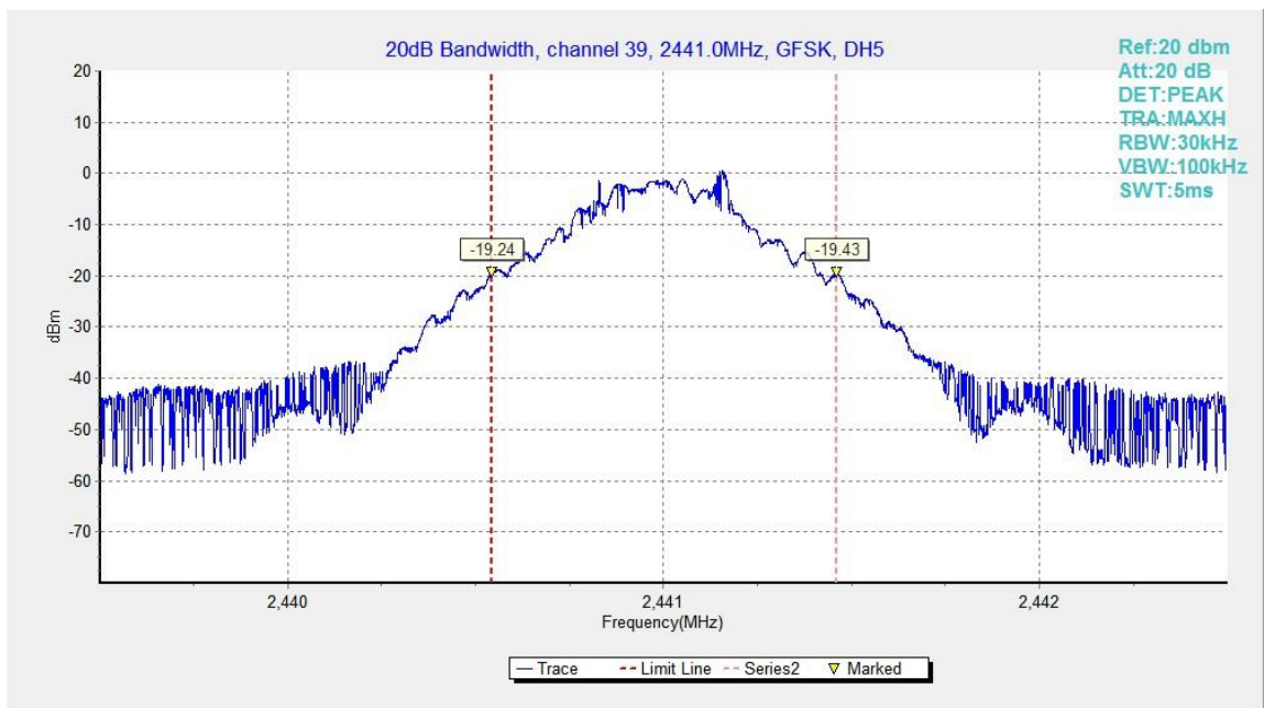
Fig.56. 20dB Bandwidth: GFSK, Channel 39
