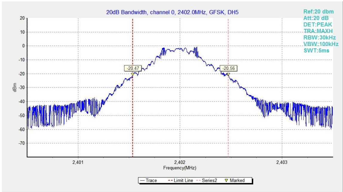
Fig.55. 20dB Bandwidth: GFSK, Channel 0
