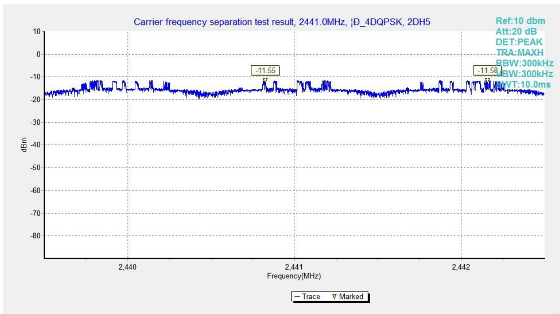
Fig.62. Carrier frequency separation measurement: \pi/4 DQPSK, Channel 39
