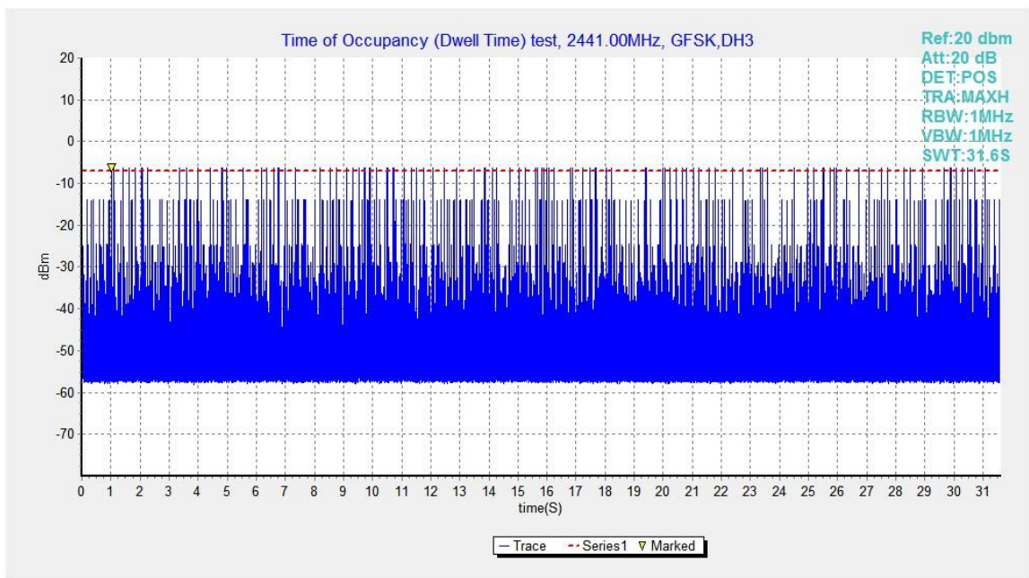
Fig.46. Number of Transmissions Measurement: Channel 39,Packet DH3
