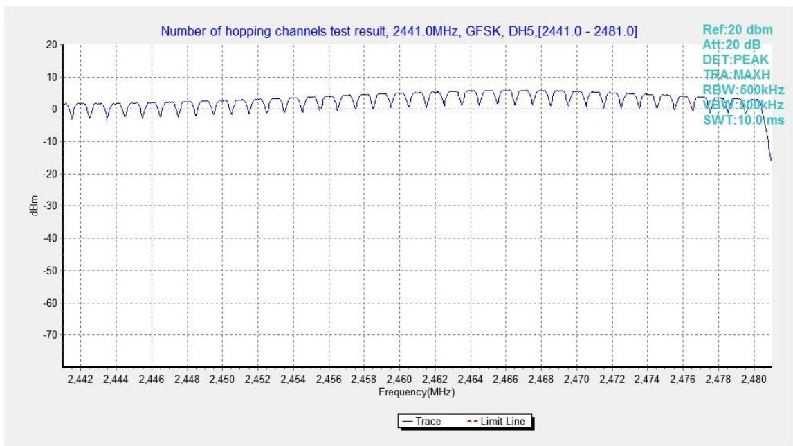
Fig.64. Number of hopping frequencies: GFSK, Channel 40 - 78
