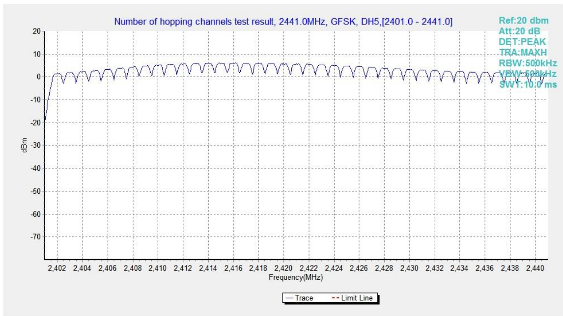
Fig.63. Number of hopping frequencies: GFSK, Channel 0 - 39
