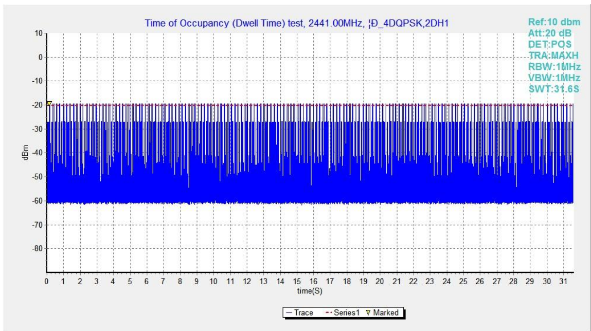
Fig.50. Number of Transmissions Measurement: Channel 39,Packet 2-DH1
