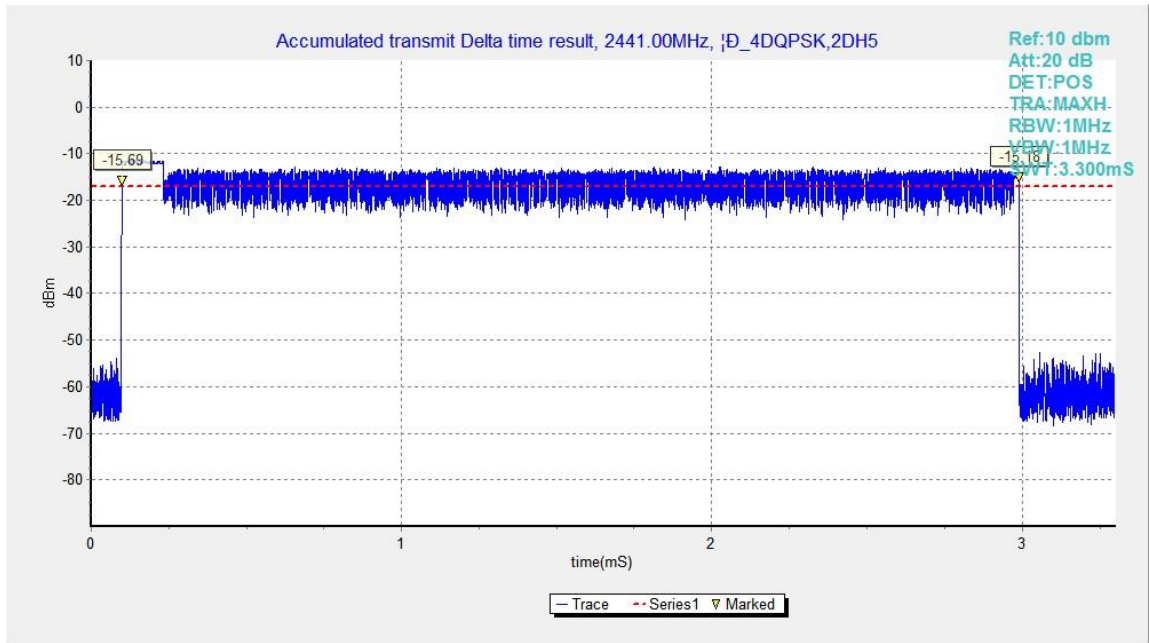
Fig.53. Time of occupancy (Dwell Time): Channel 39, Packet 2-DH5
