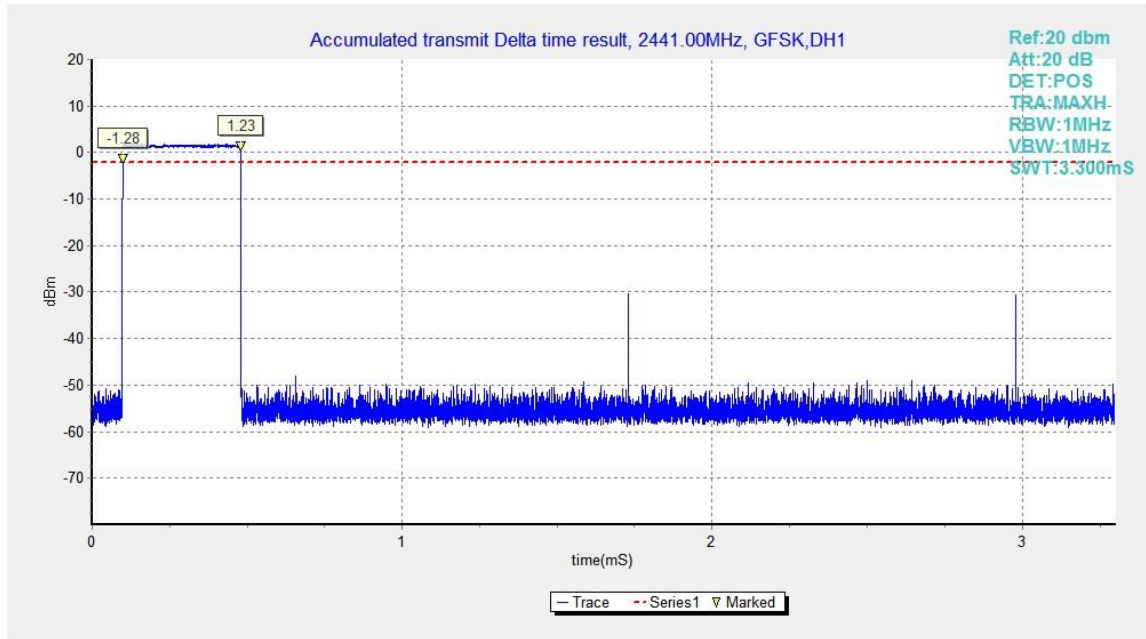
Fig.43. Time of occupancy (Dwell Time): Channel 39, Packet DH1
