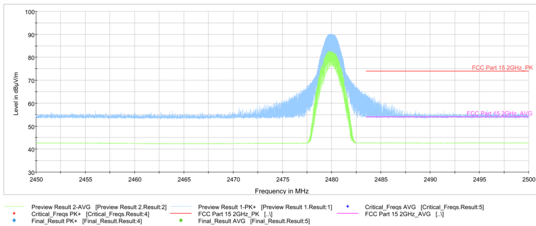
Fig.12. Frequency Band Edges: \pi/4 DQPSK, Channel 78, Hopping Off, 2.45 GHz - 2.50GHz
