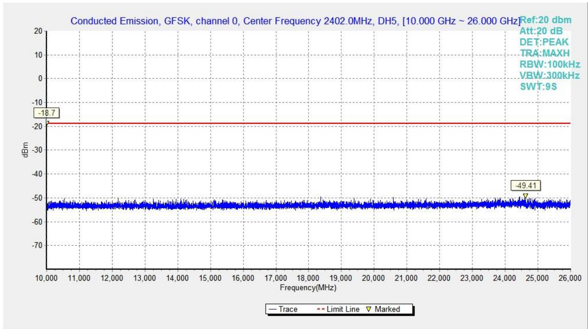
Fig.17. Conducted spurious emission: GFSK, Channel 0, 10GHz - 26GHz
