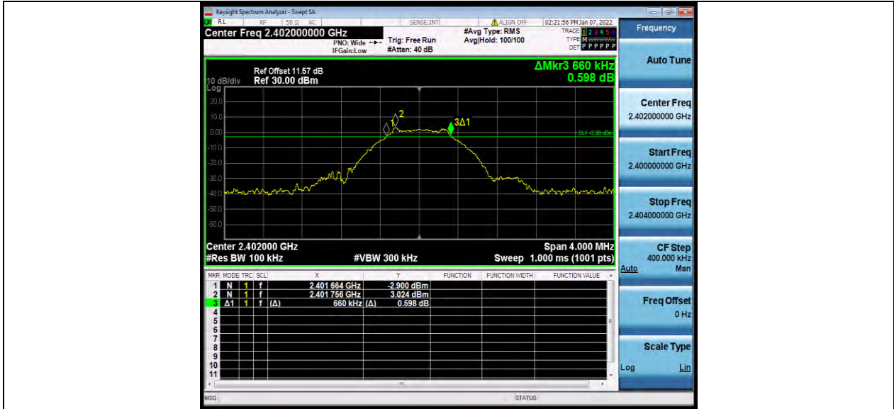
BLE_1M_Ant1_2402
