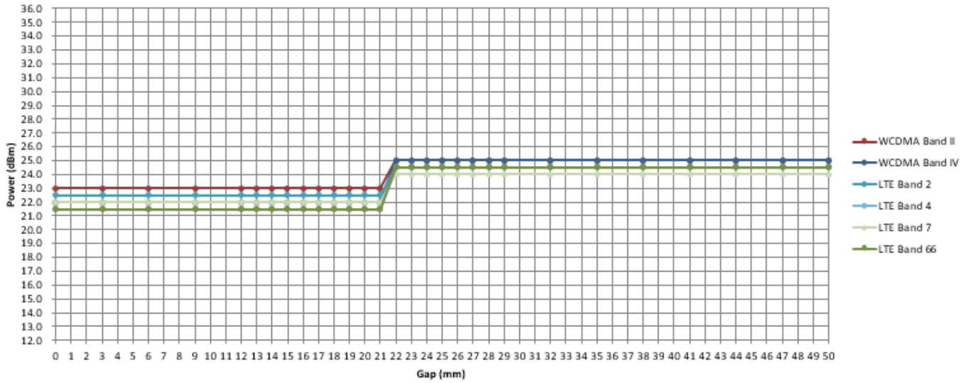
Output Power Verification in dBm for EUT Bottom Side (moving toward phantom)
