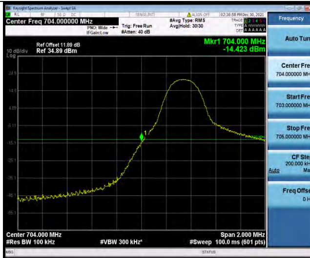
Band17-5MHz-QPSK-23755-25RB#0
