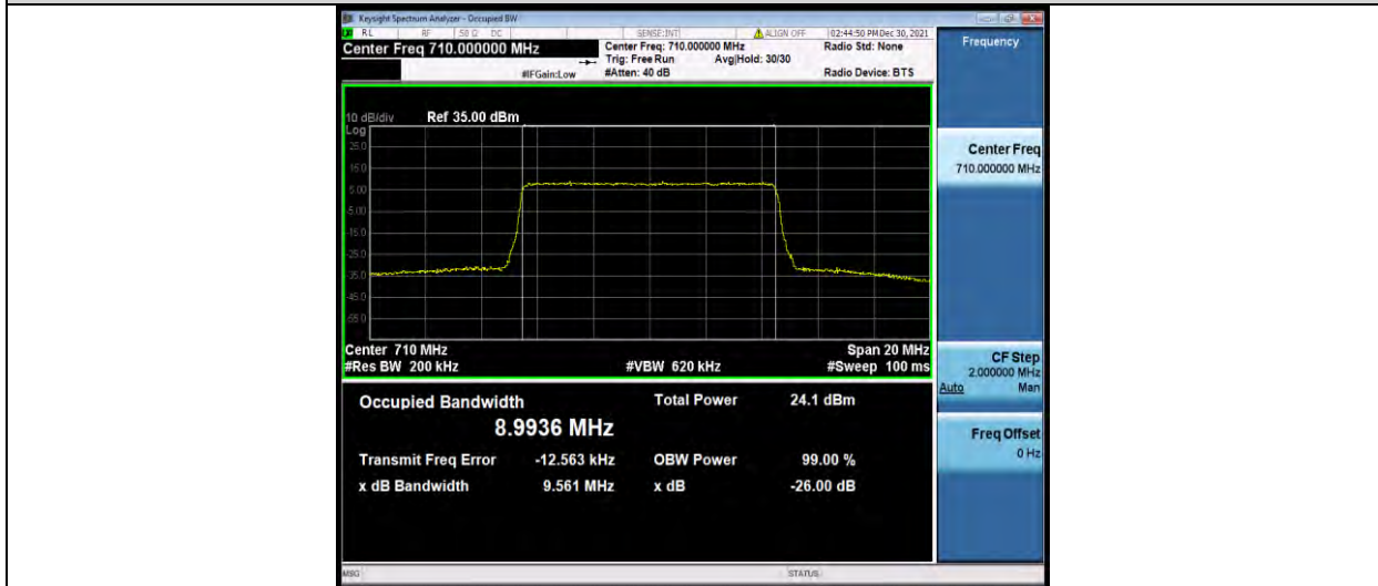
Band17-10MHz-QPSK-23800-50RB#0
