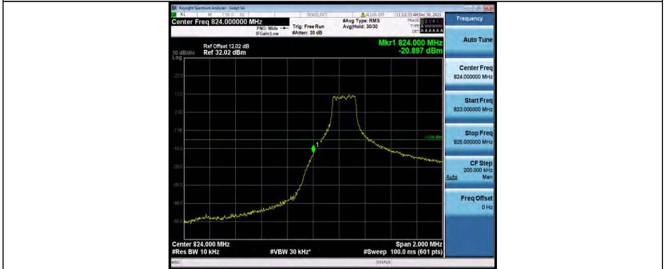
Band5-3MHz-16QAM-20415-15RB#0
