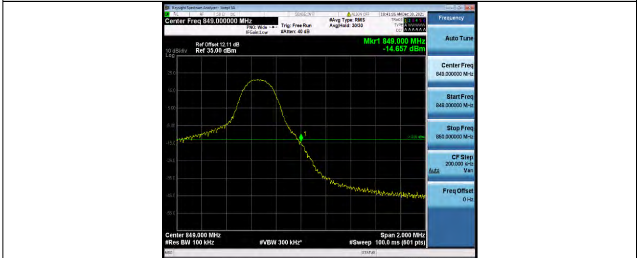
Band5-5MHz-QPSK-20625-25RB#0
