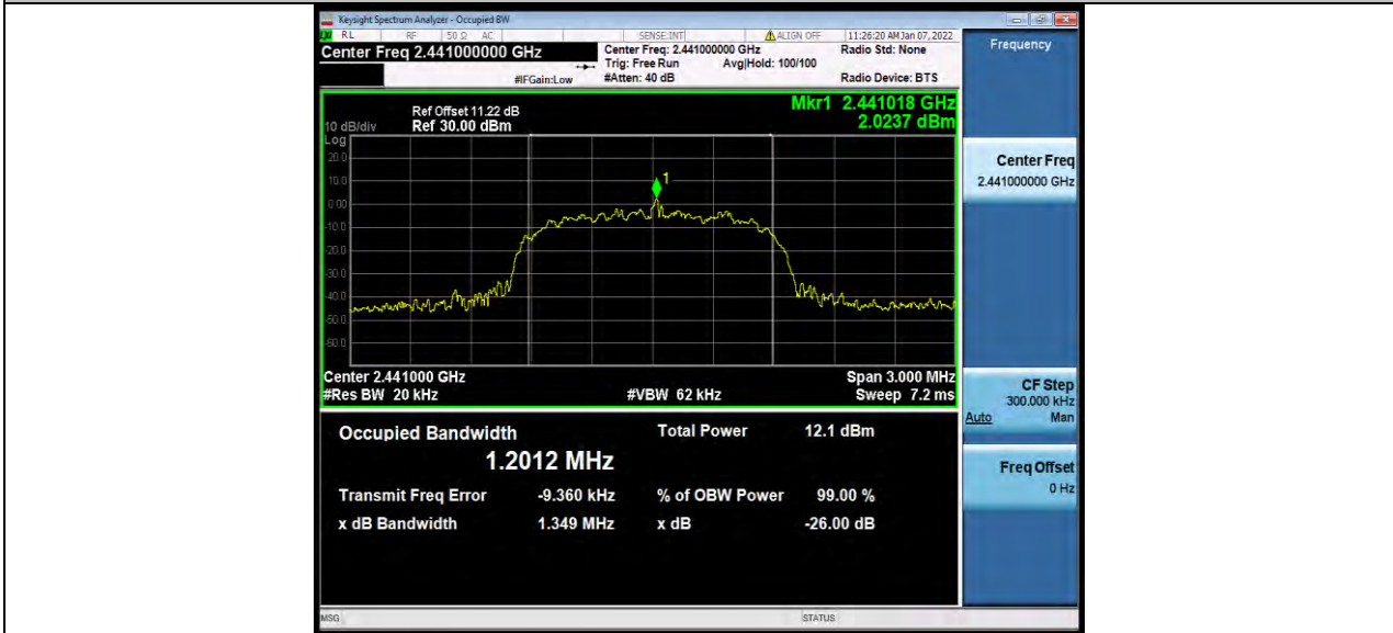
3DH5_Ant1_2441
