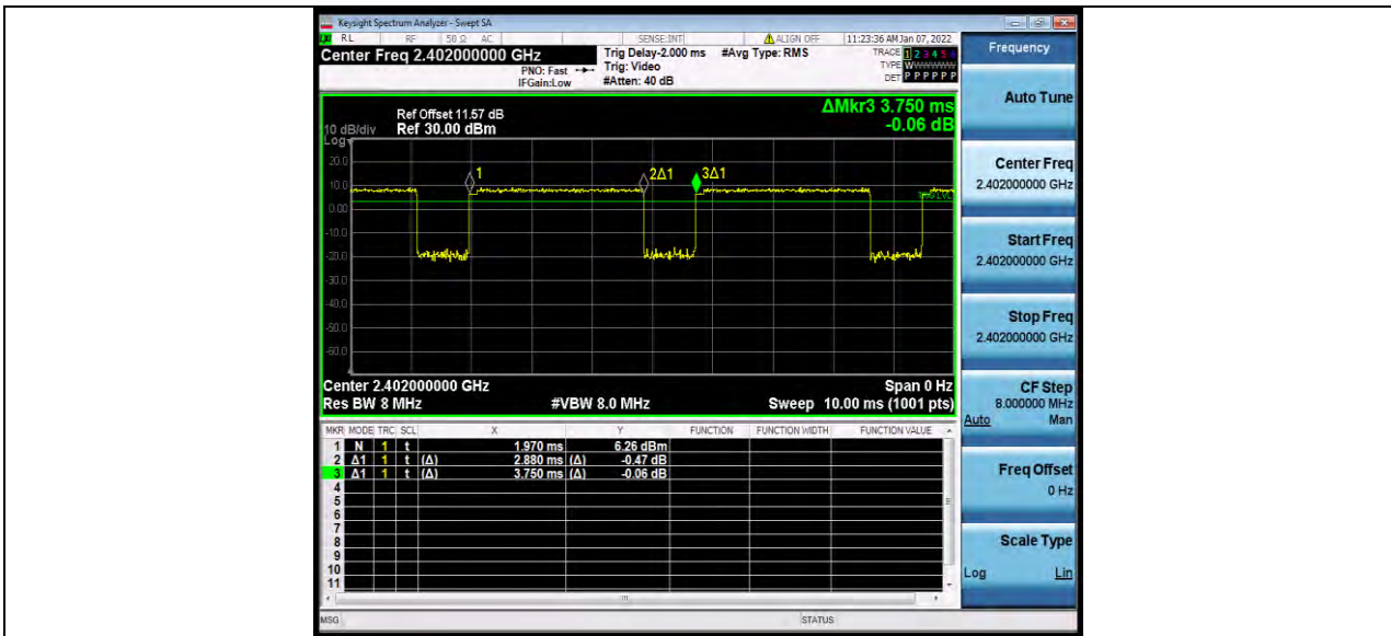
3DH5_Ant1_2402
