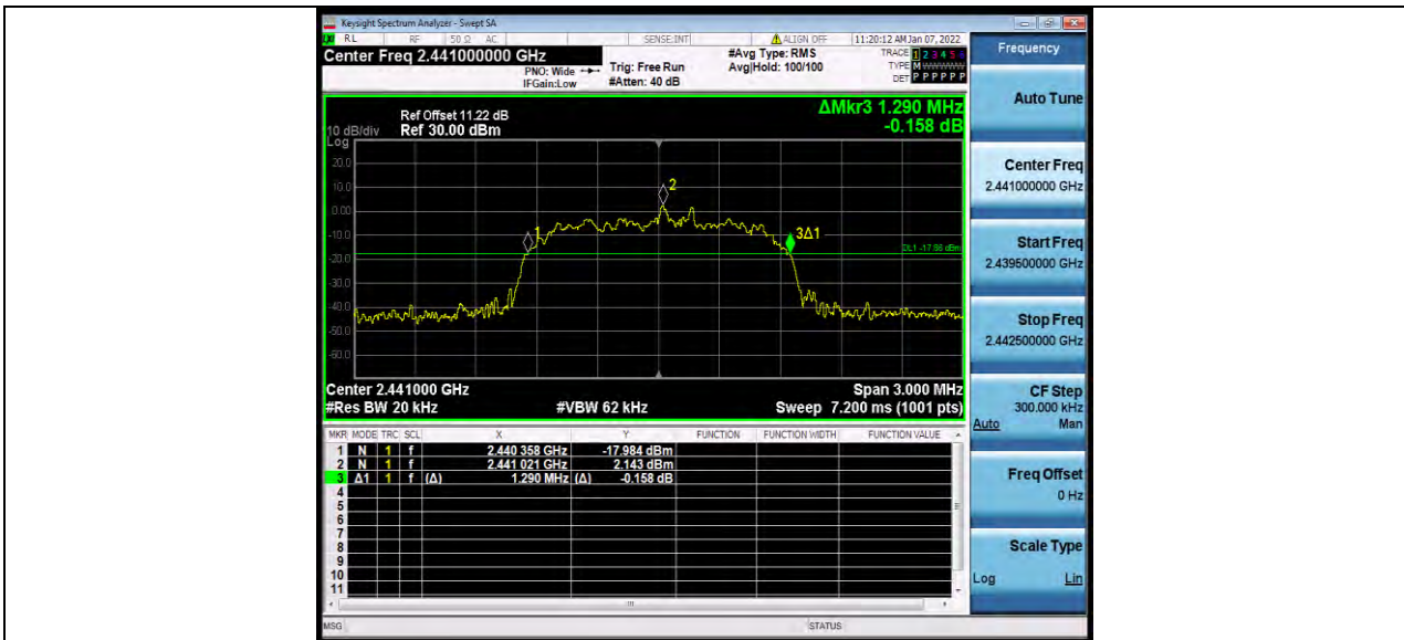
2DH5_Ant1_2441
