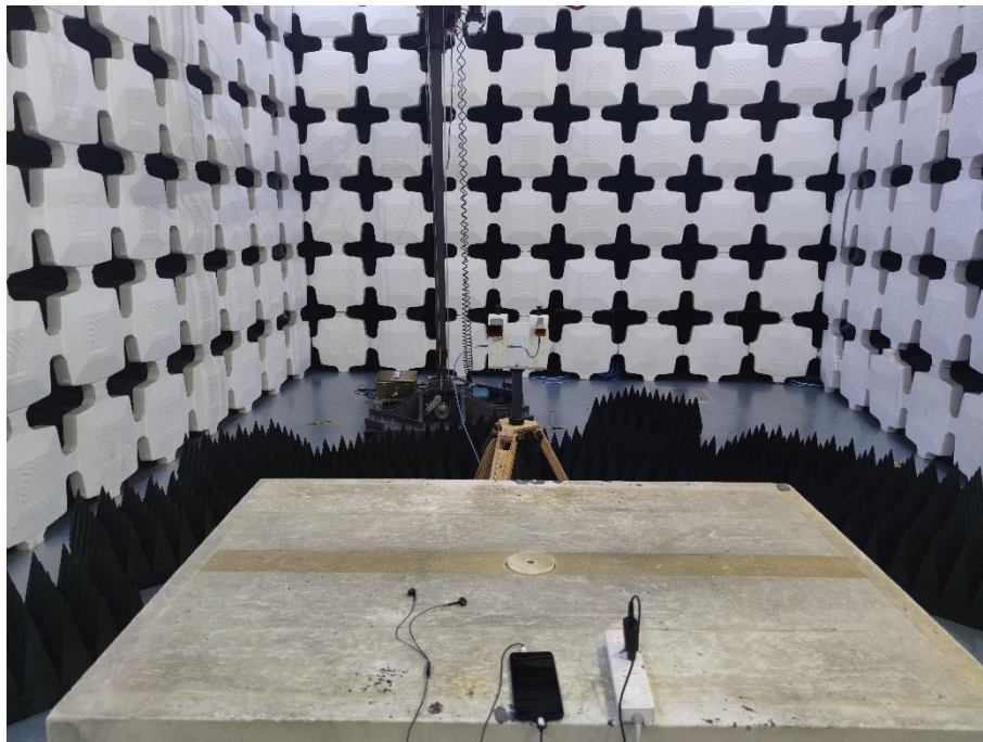
4. Radiated Emissions (Part 15B, Video Player, 26GHz-40GHz)
