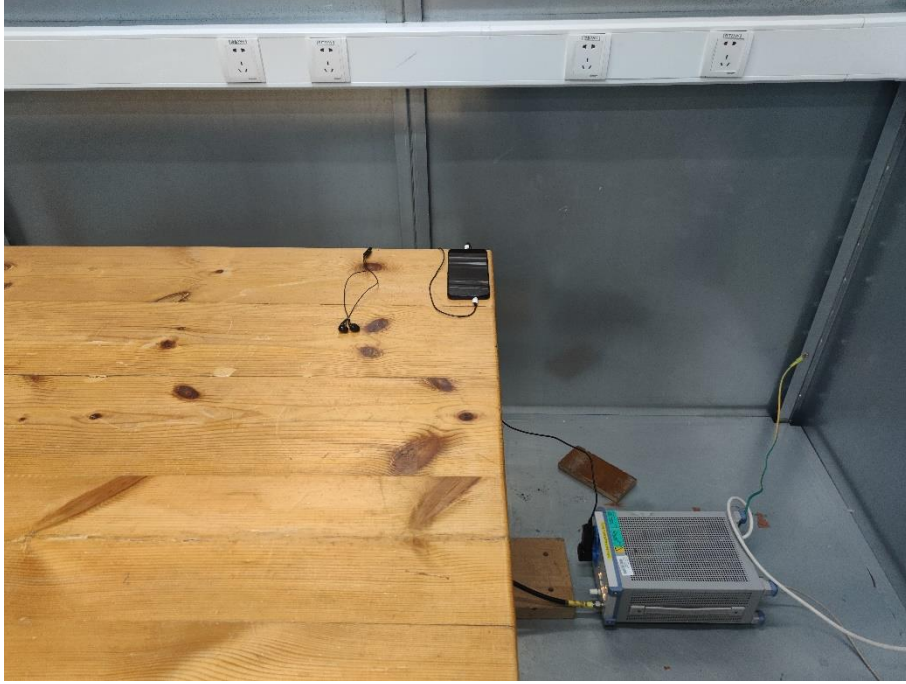
5. Conducted Emission (Part 15B, FM receive)
