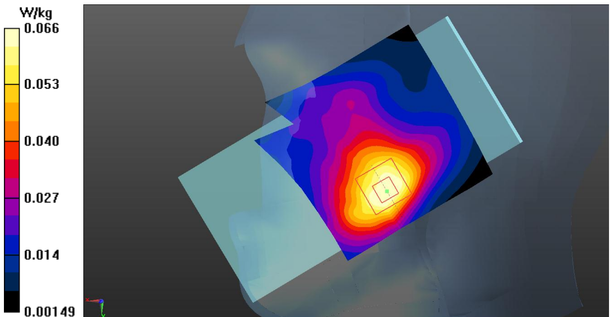
Fig.3 PCS1900 Head
