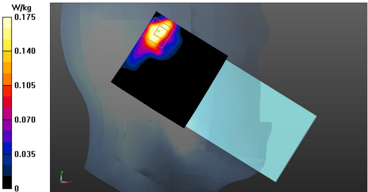
Fig.29 WLAN 5GHz Head
