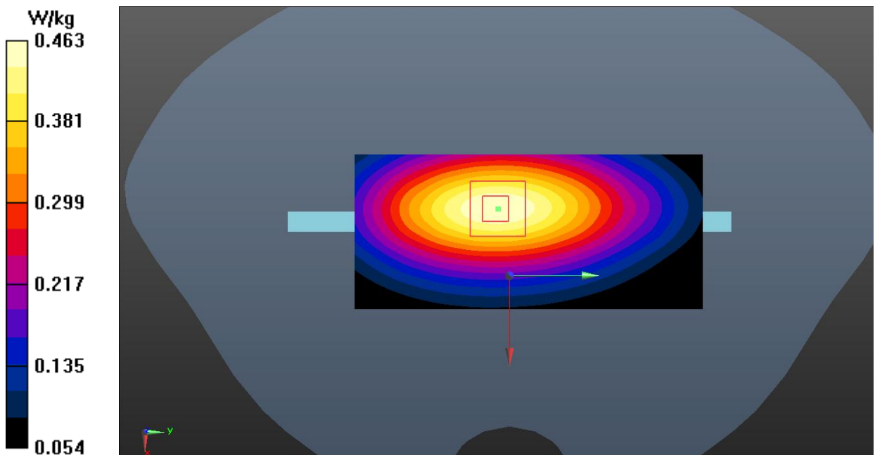
Fig.22 LTE Band 28 Body
