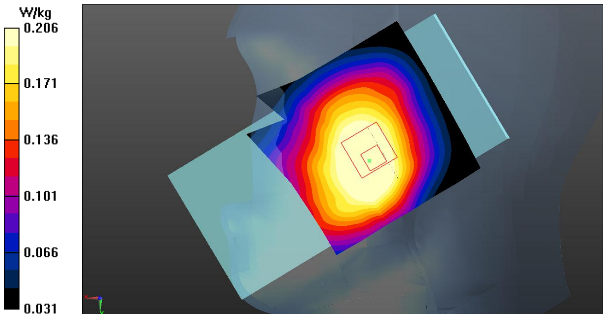
Fig.21 LTE Band 28 Head
