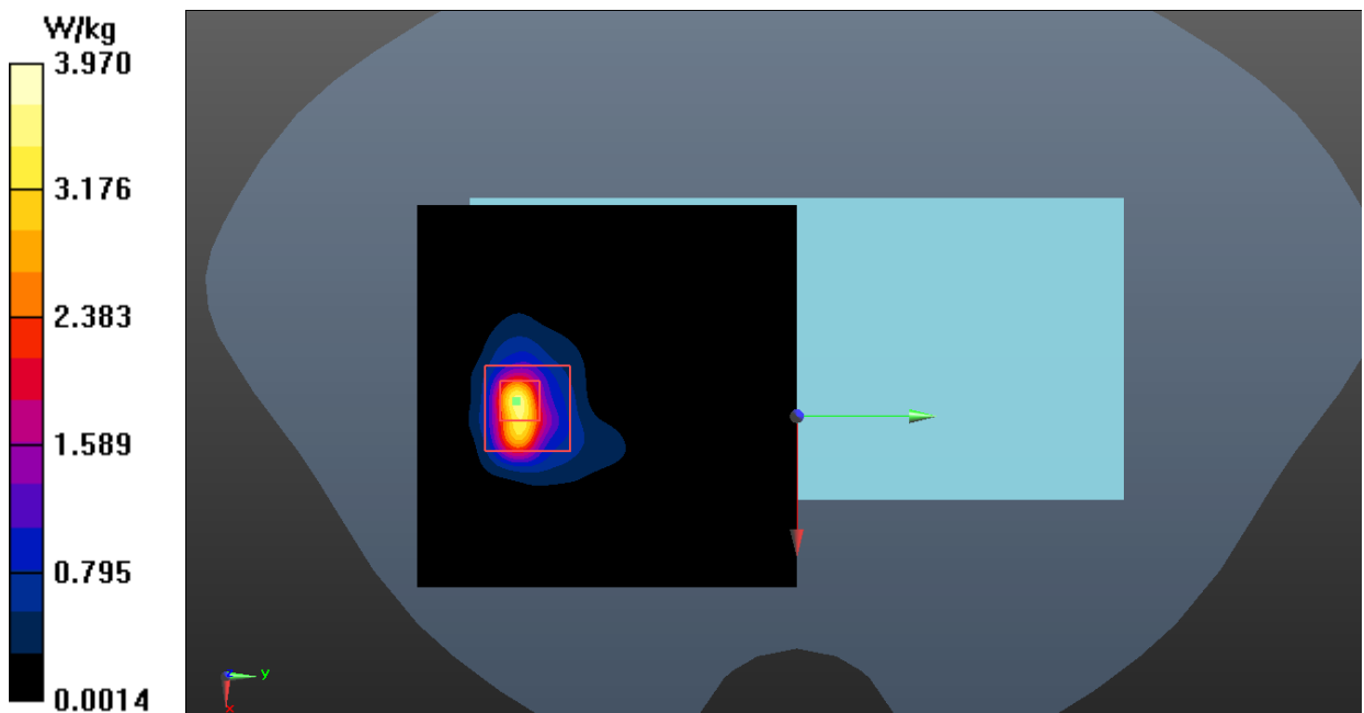
Fig.31 WLAN 5GHz Extremity
