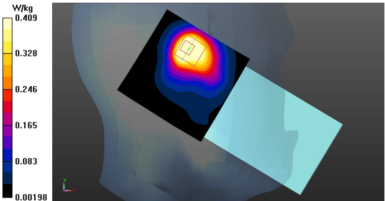
Fig.27 WLAN 2.4GHz Head
