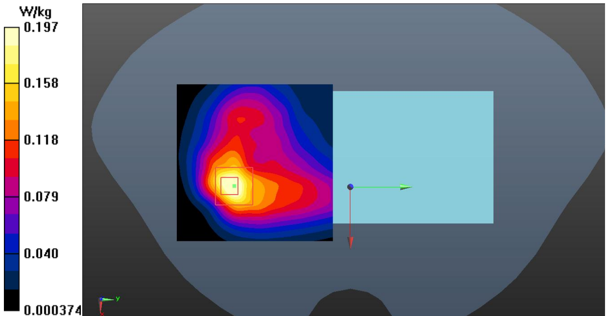
Fig.28 WLAN 2.4GHz Body
