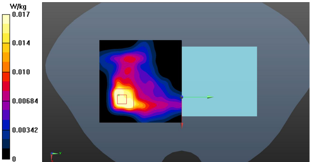
Fig.26 Bluetooth Body
