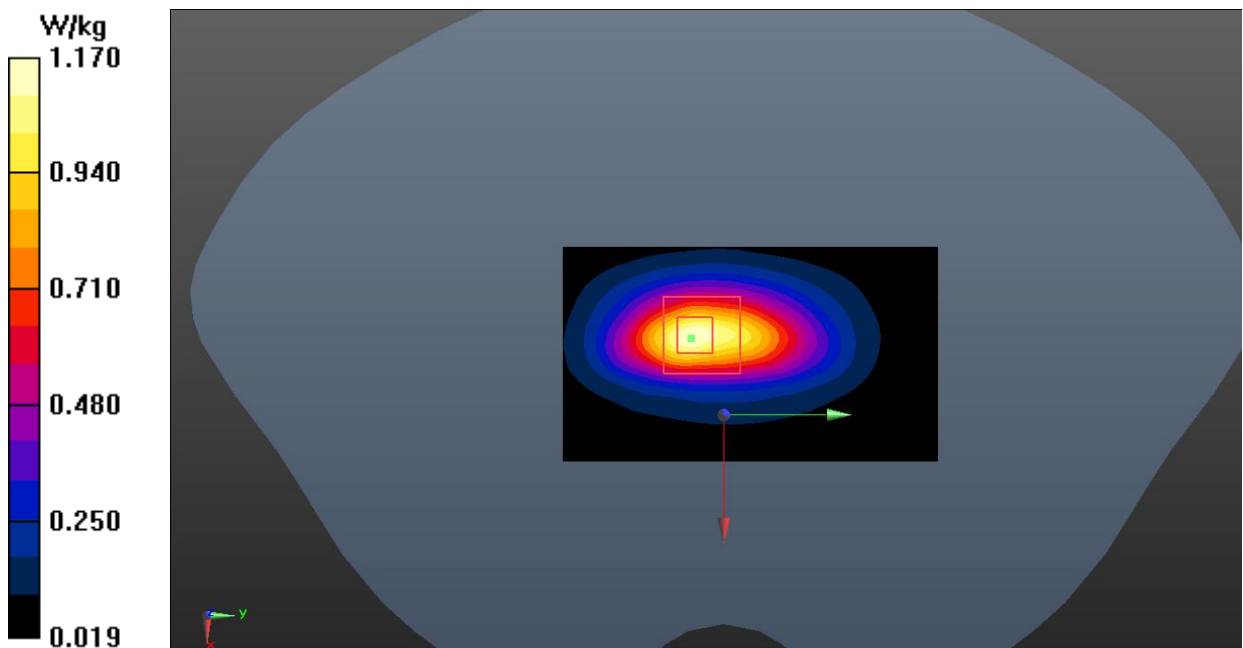
Fig.4 PCS1900 Body
