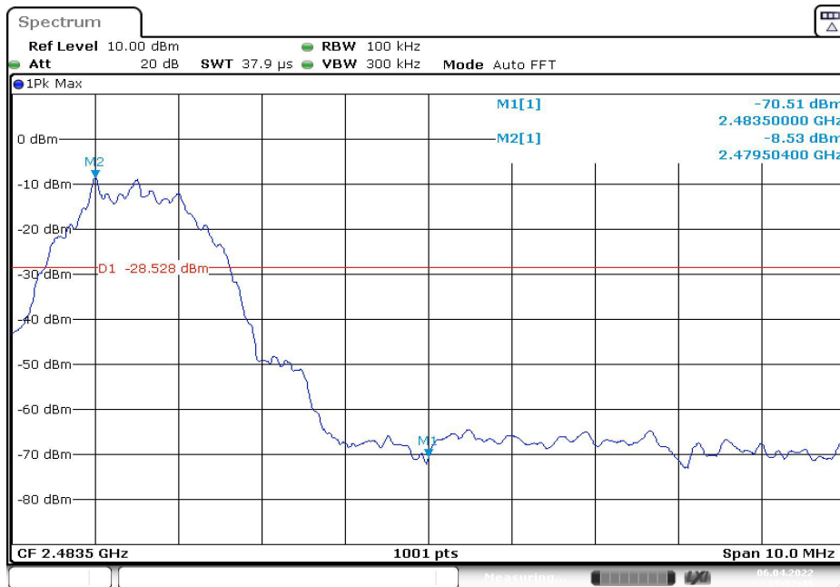
Fig.16 Band Edges (Ch 39), LE 2M
