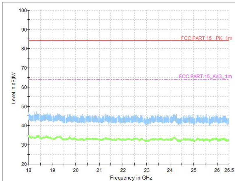
Fig. 39 Radiated Spurious Emission (All Channels, 18 GHz ~26.5 GHz)
