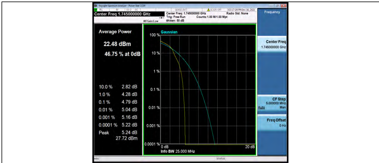
Band66-1.4MHz-16QAM-132322-6RB#0
