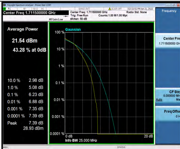
Band66-3MHz-64QAM-132322-1RB#0
