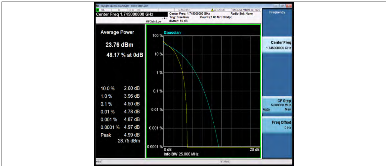
Band66-20MHz-QPSK-132322-100RB#0
