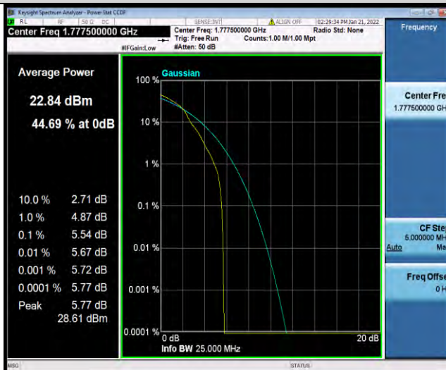
Band66-5MHz-64QAM-132647-25RB#0
