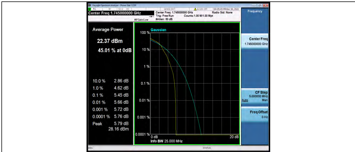
Band66-10MHz-16QAM-132322-50RB#0
