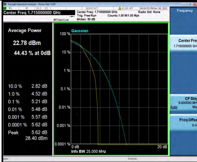
Band66-10MHz-16QAM-132022-50RB#0
