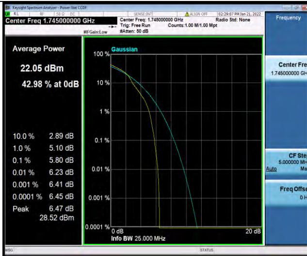
Band66-5MHz-64QAM-132322-25RB#0
