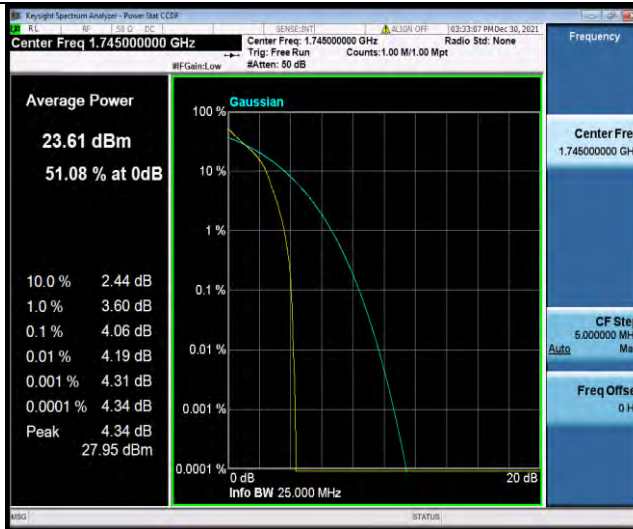
Band66-3MHz-QPSK-132322-15RB#0
