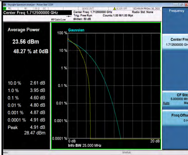
Band66-5MHz-QPSK-131997-25RB#0
