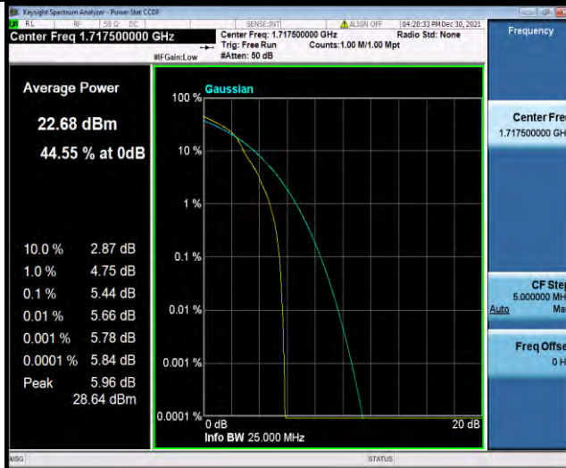
Band66-15MHz-16QAM-132047-75RB#0
