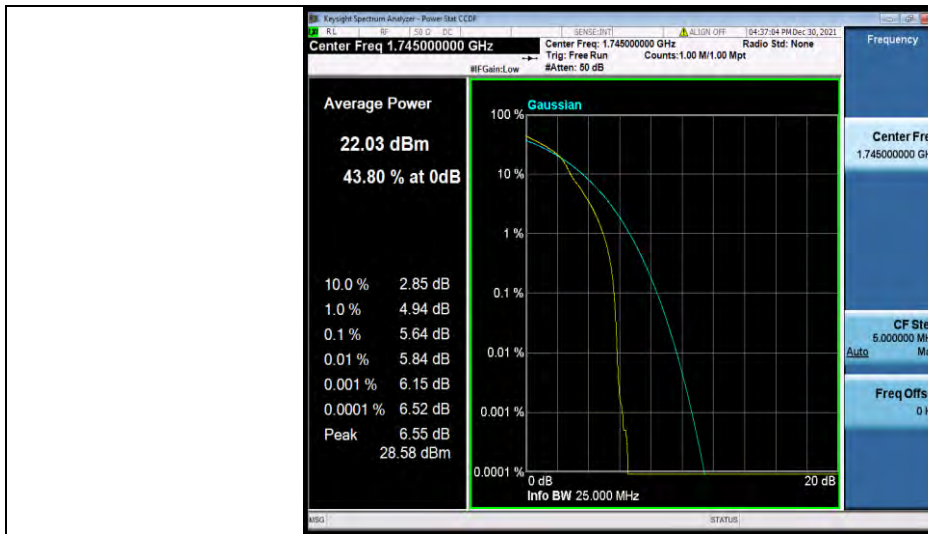
Band66-20MHz-16QAM-132322-100RB#0
