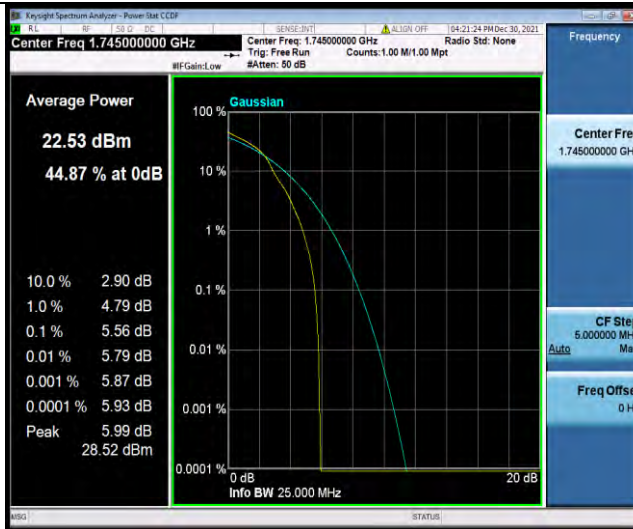
Band66-15MHz-16QAM-132322-75RB#0
