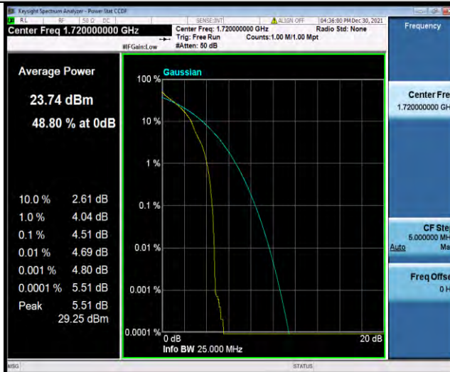
Band66-20MHz-QPSK-132072-100RB#0
