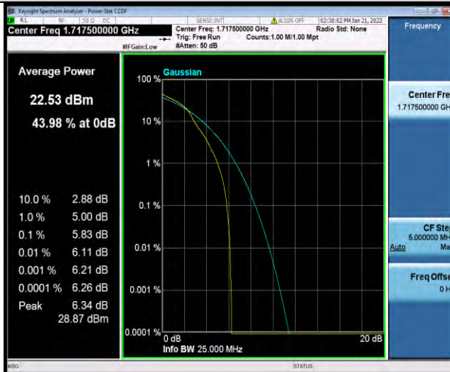
Band66-15MHz-64QAM-132047-75RB#0
