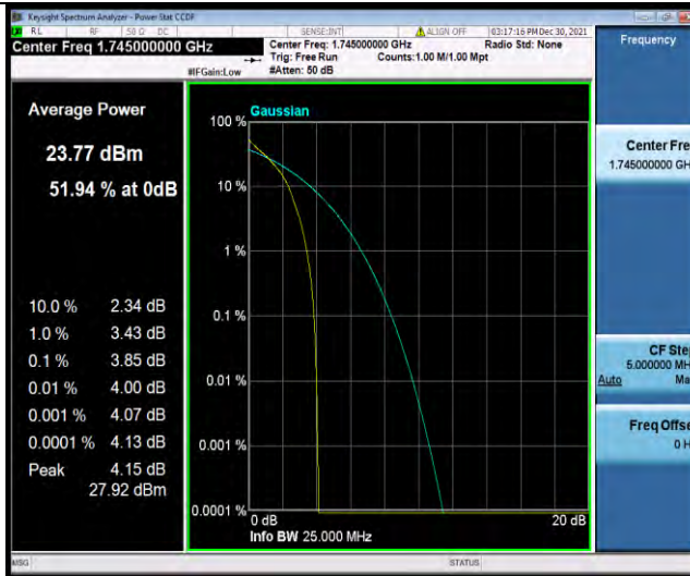
Band66-1.4MHz-QPSK-132322-6RB#0
