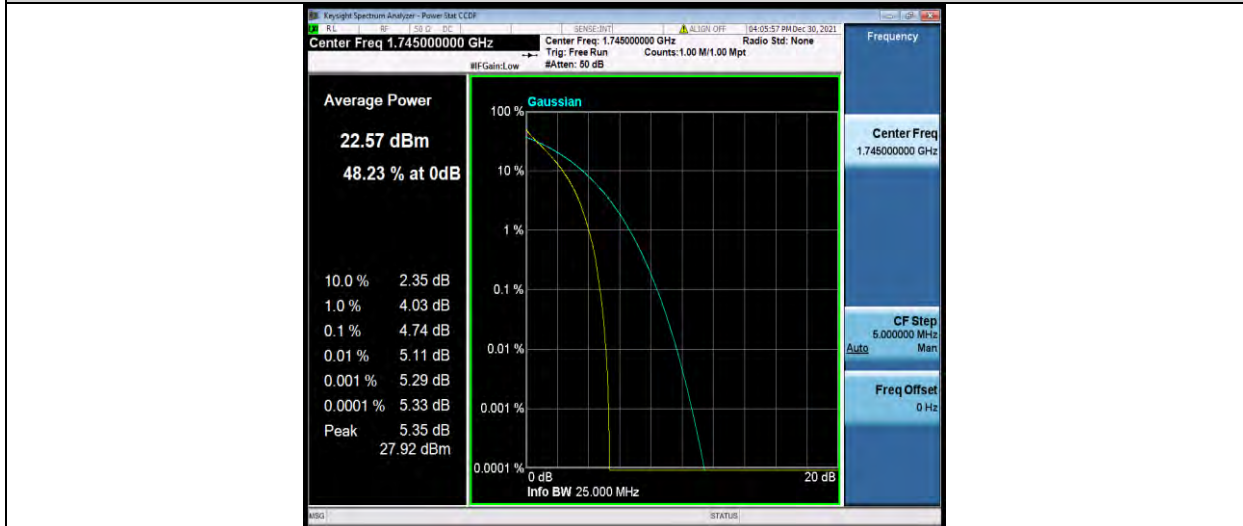
Band66-10MHz-QPSK-132622-1RB#0
