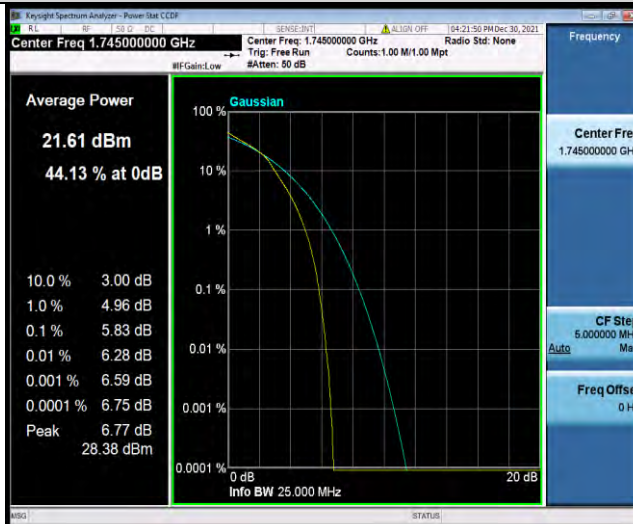
Band66-15MHz-16QAM-132597-1RB#0
