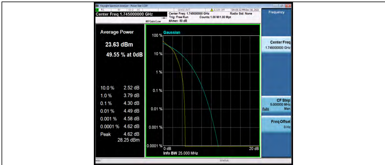
Band66-10MHz-QPSK-132322-50RB#0
