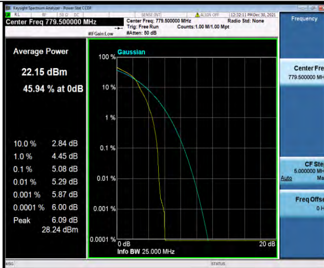
Band13-5MHz-16QAM-23205-25RB#0
