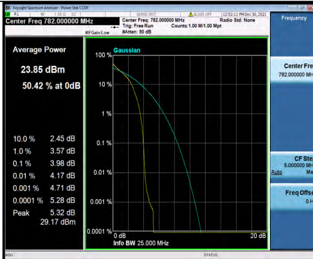
Band13-10MHz-QPSK-23230-50RB#0
