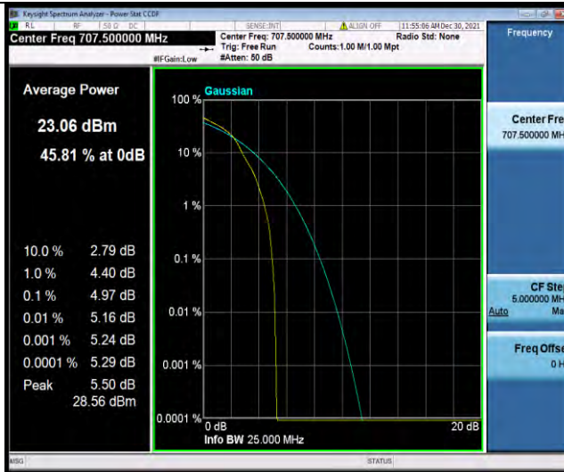
Band12-10MHz-16QAM-23095-50RB#0
