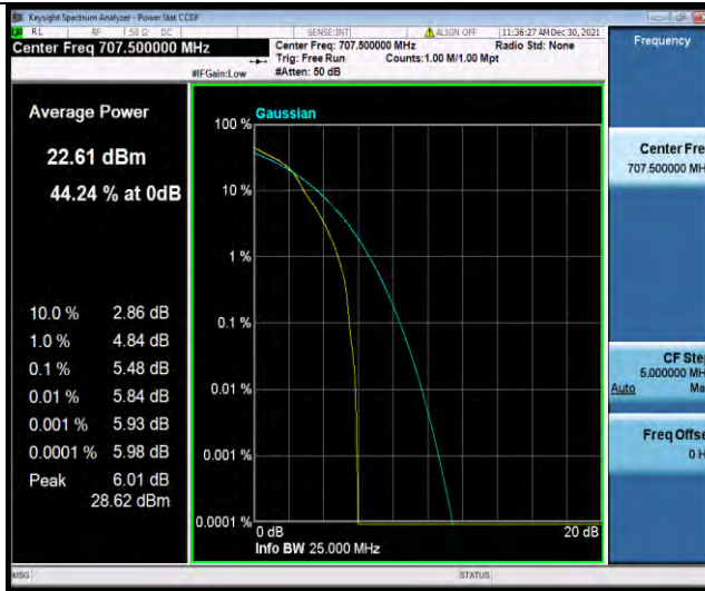
Band12-3MHz-16QAM-23095-15RB#0
