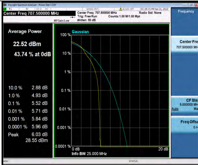
Band12-10MHz-64QAM-23095-50RB#0
