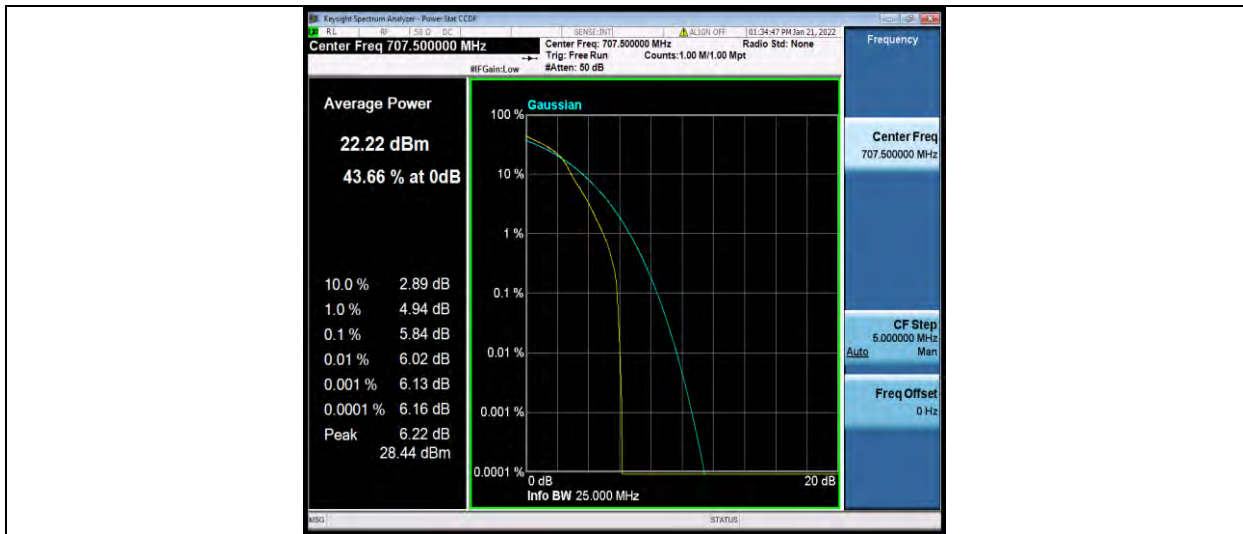
Band12-5MHz-64QAM-23095-25RB#0
