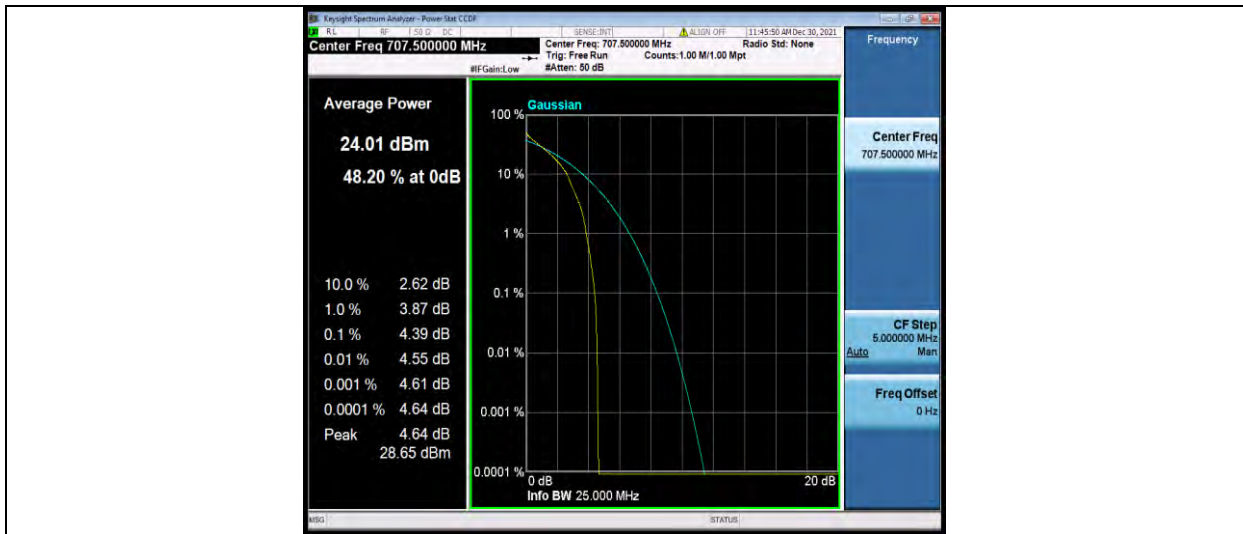
Band12-5MHz-QPSK-23095-25RB#0
