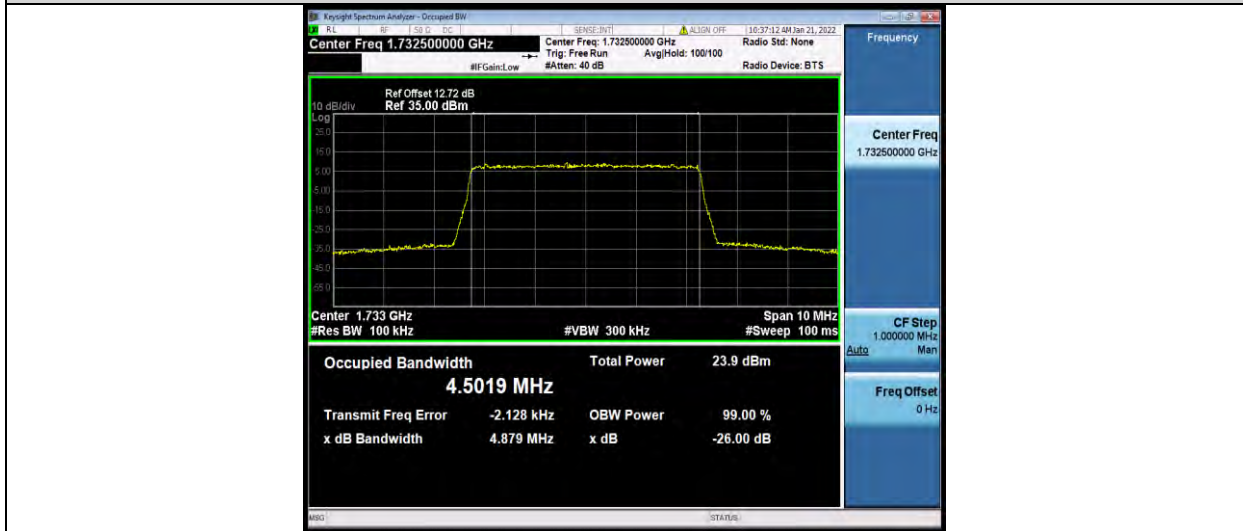
Band4-5MHz-64QAM-20375-25RB#0
