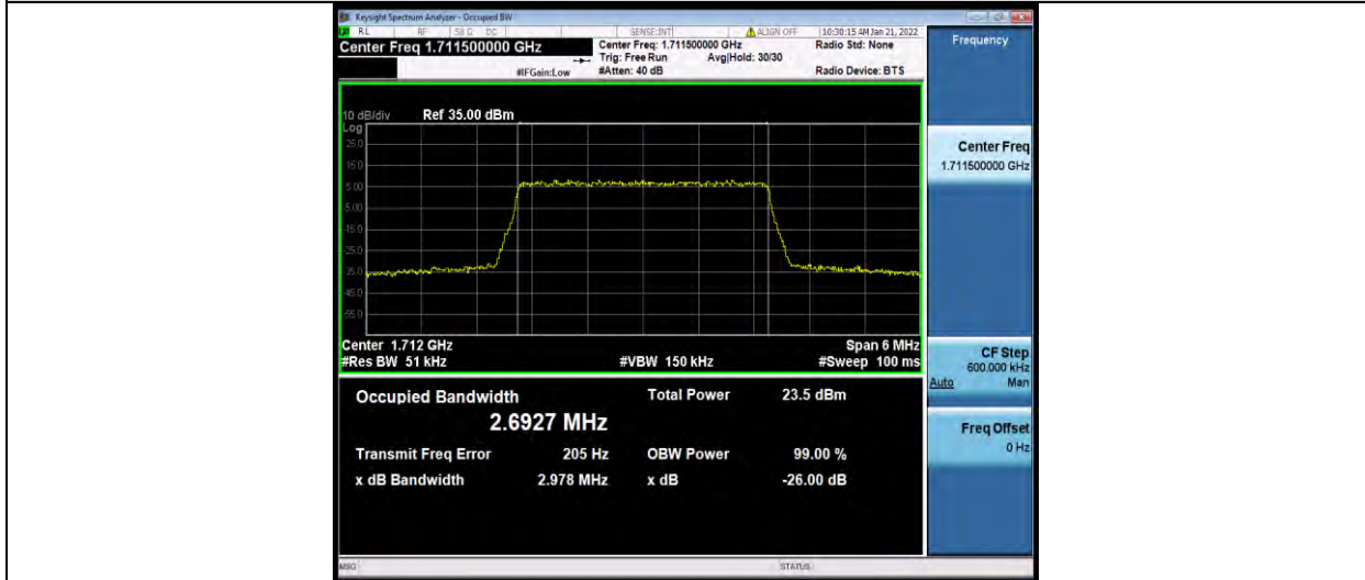
Band4-3MHz-64QAM-20175-15RB#0
