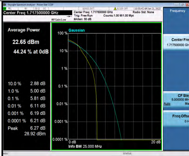
Band4-15MHz-64QAM-20025-75RB#0
