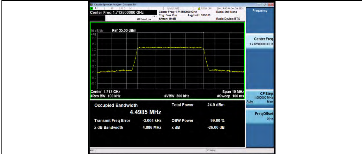
Band4-5MHz-QPSK-20175-25RB#0
