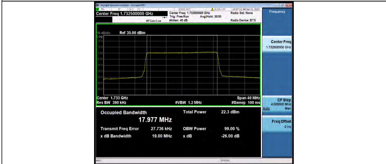
Band4-20MHz-64QAM-20300-100RB#0
