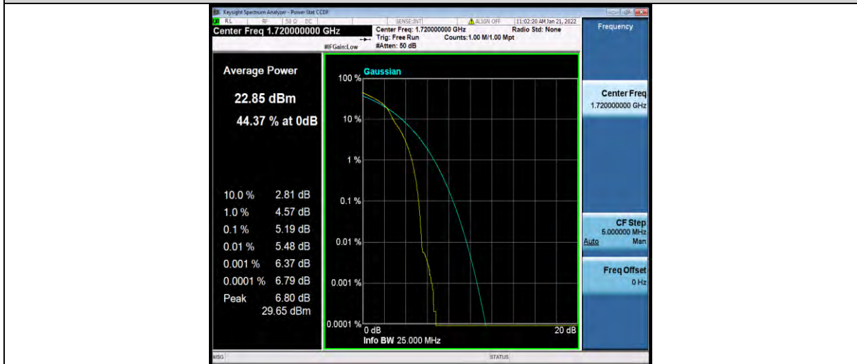
Band4-20MHz-64QAM-20050-100RB#0
