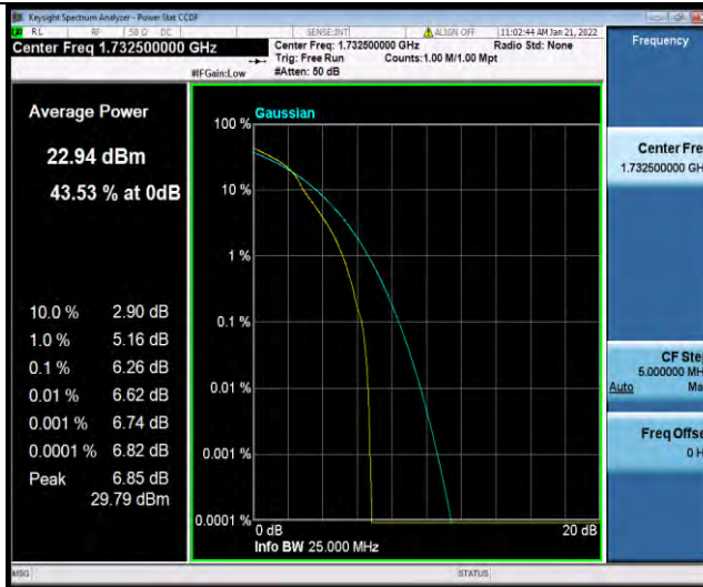
Band4-20MHz-64QAM-20175-100RB#0
