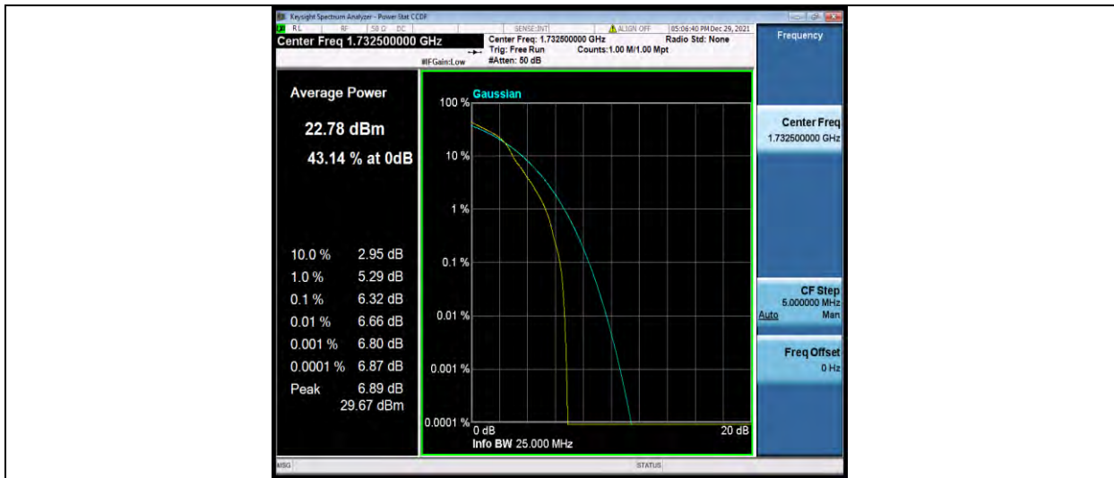
Band4-20MHz-16QAM-20175-100RB#0
