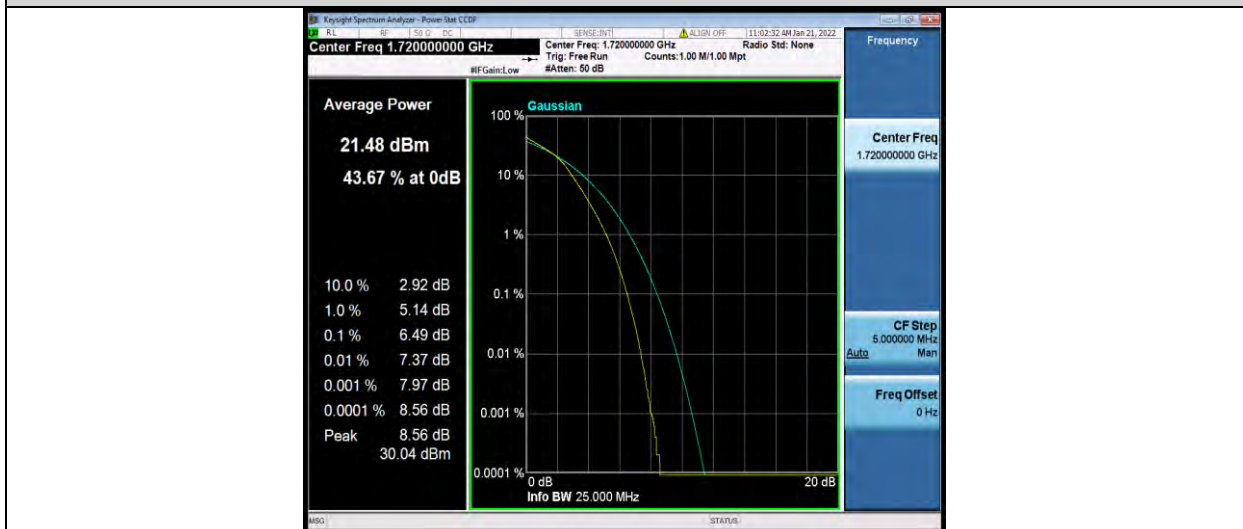
Band4-20MHz-64QAM-20175-1RB#0
