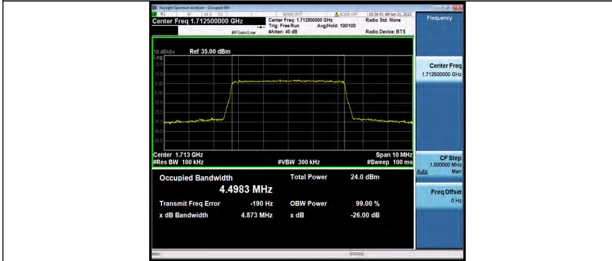
Band4-5MHz-64QAM-20175-25RB#0
