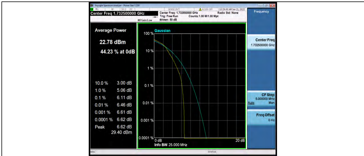
Band4-1.4MHz-64QAM-20175-6RB#0
