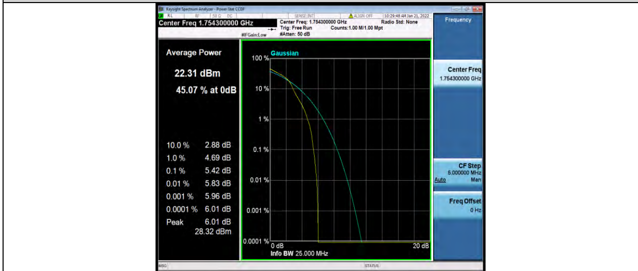
Band4-1.4MHz-64QAM-20393-6RB#0
