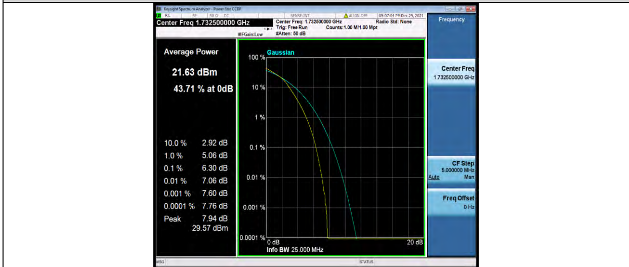
Band4-20MHz-16QAM-20300-1RB#0
