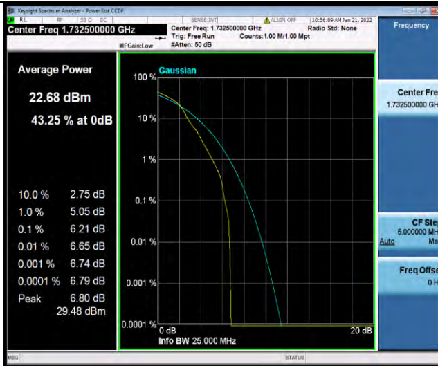
Band4-15MHz-64QAM-20175-75RB#0
