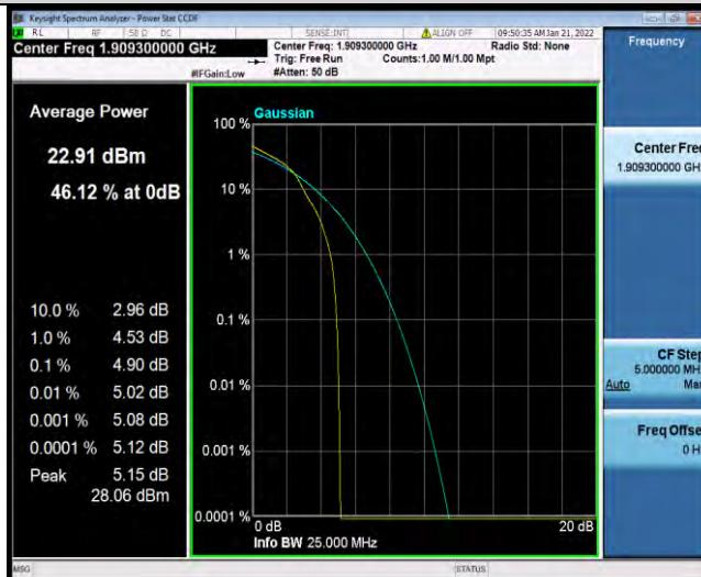
Band2-1.4MHz-64QAM-19193-6RB#0
