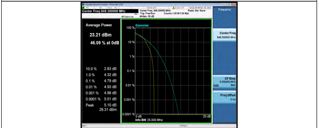
Band5-1.4MHz-16QAM-20643-6RB#0
