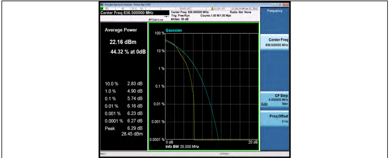
Band5-1.4MHz-64QAM-20525-6RB#0
