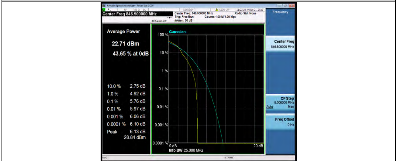
Band5-5MHz-64QAM-20625-25RB#0
