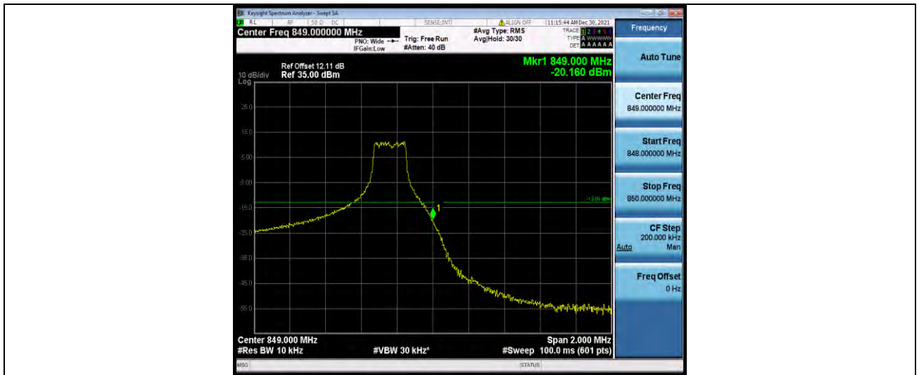
Band5-3MHz-16QAM-20635-15RB#0
