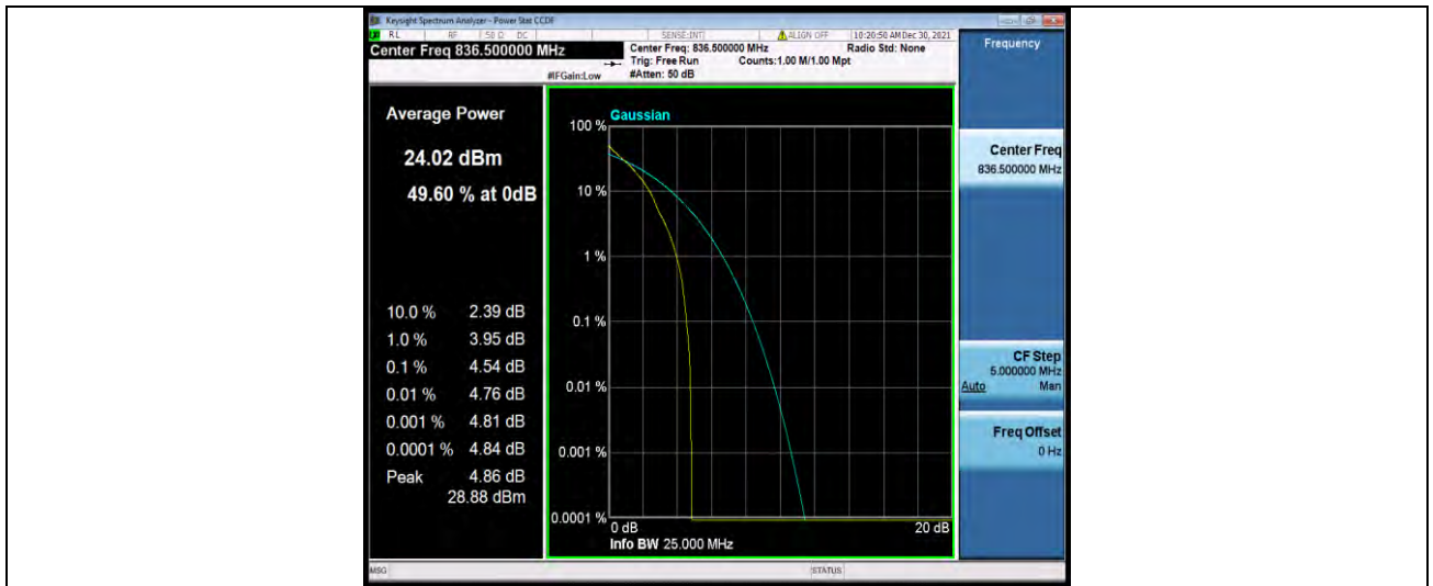
Band5-1.4MHz-QPSK-20525-6RB#0
