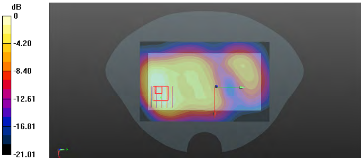
0 dB = 0.600 W/kg
