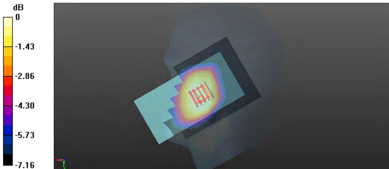
0 dB = 0.205 W/kg
