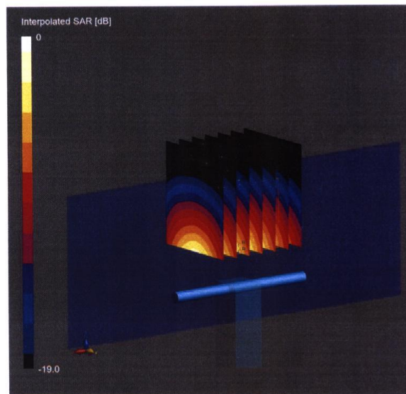
0 dB = 29.3 W/Kg
