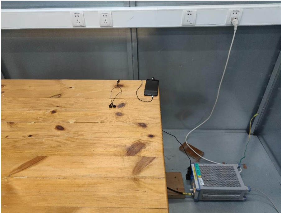
5. Conducted Emission (Part 15B, Video Player/FM receive)
