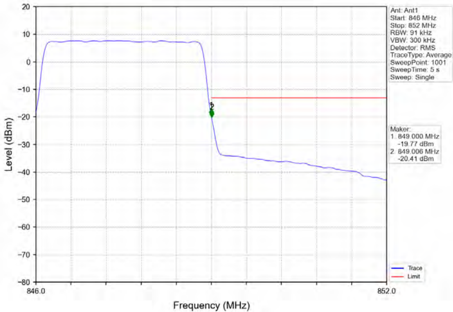
Band5_3MHz_16QAM_HCH_847.5MHz_RB_15_0_NTNV
