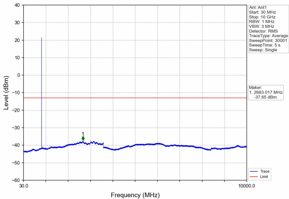
Band5_1.4MHz_64QAM_MCH_836.5MHz_RB_1_0_NTNV
