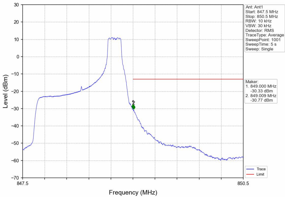
Band5_1.4MHz_16QAM_HCH_848.3MHz_RB_6_0_NTNV
