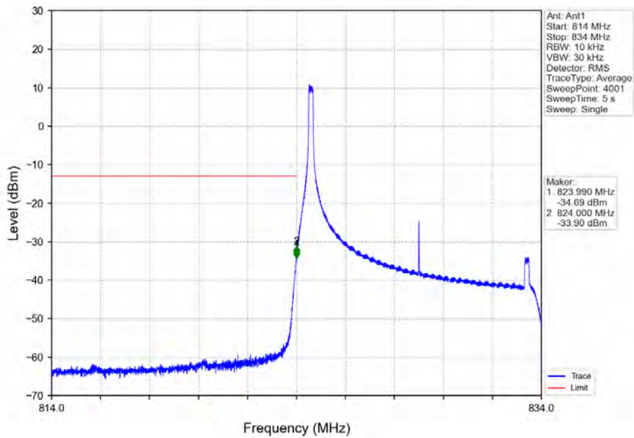
Band5 10MHz 64QAM LCH 829MHz RB 1 0 NTV
