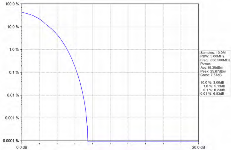
Band5 10MHz 64QAM MCH 836.5MHz RB 50 0 NTV
