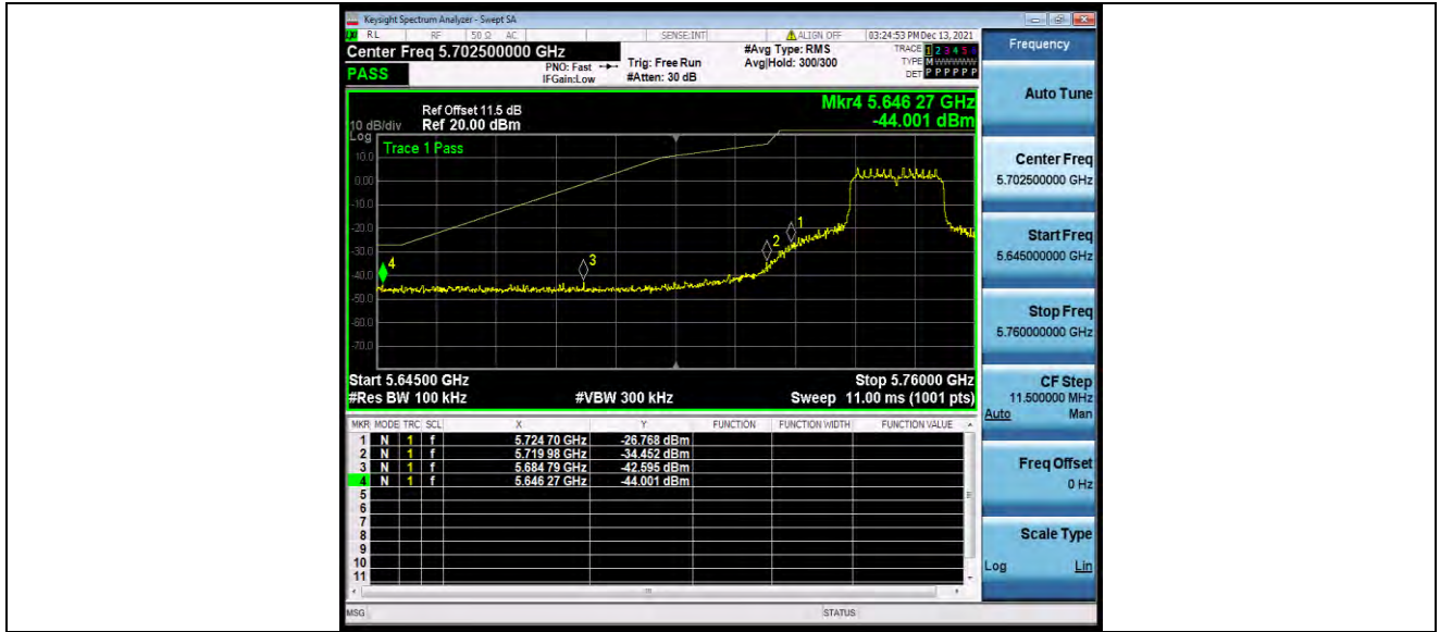
11N20SISO_Ant1_Low_5745
