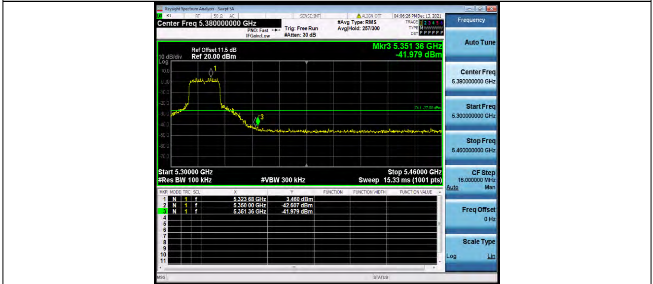
11AC20SISO_Ant1_High_5320
