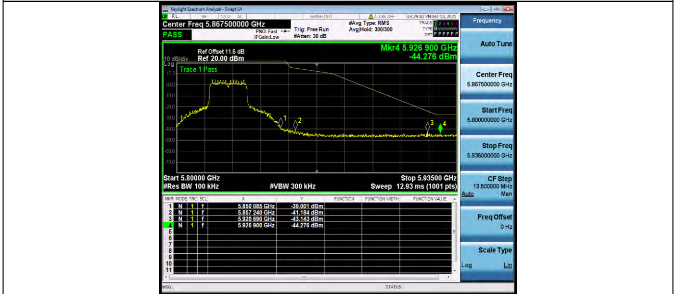
11N20SISO_Ant1_High_5825
