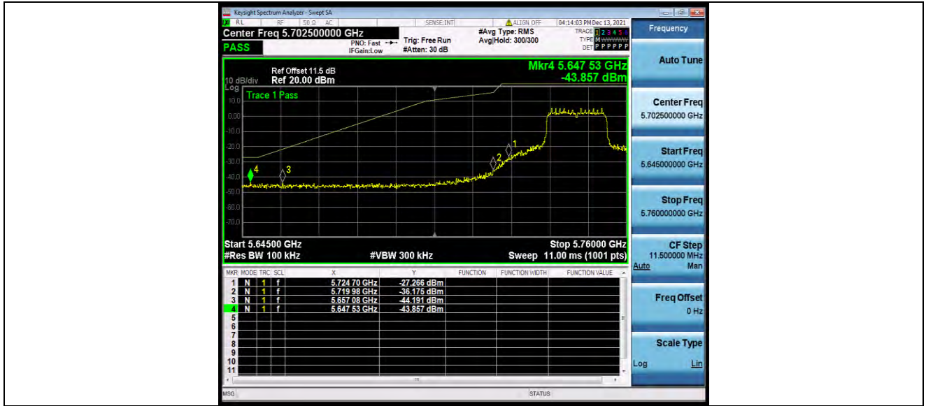
11AC20SISO_Ant1_Low_5745
