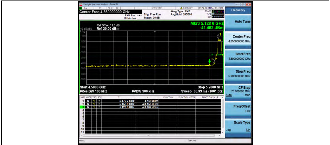
11AC20SISO_Ant1_Low_5180
