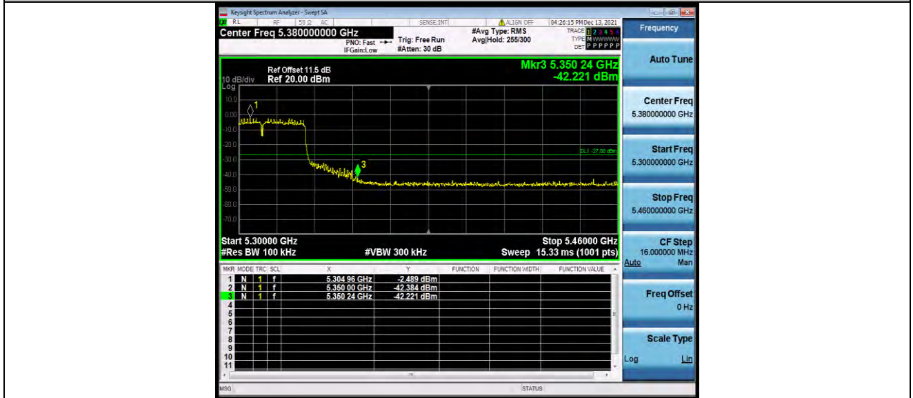
11AC40SISO_Ant1_High_5310
