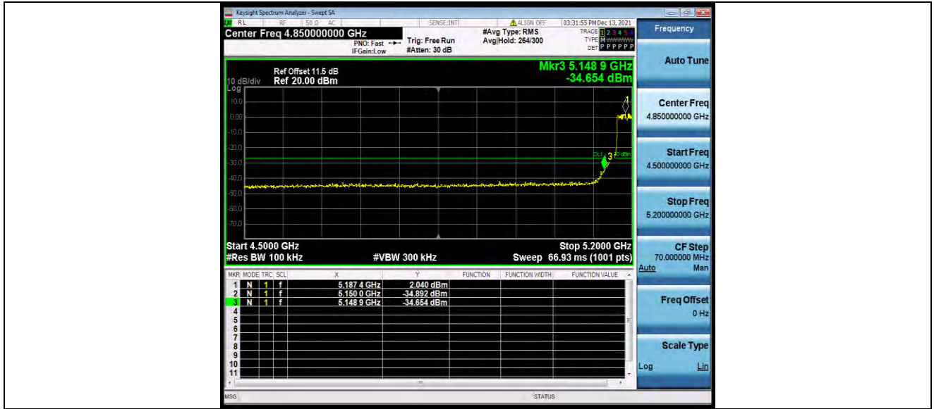
11N40SISO_Ant1_Low_5190
