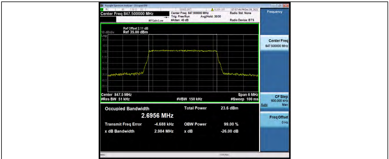
Band5-3MHz-64QAM-20415-15RB#0
