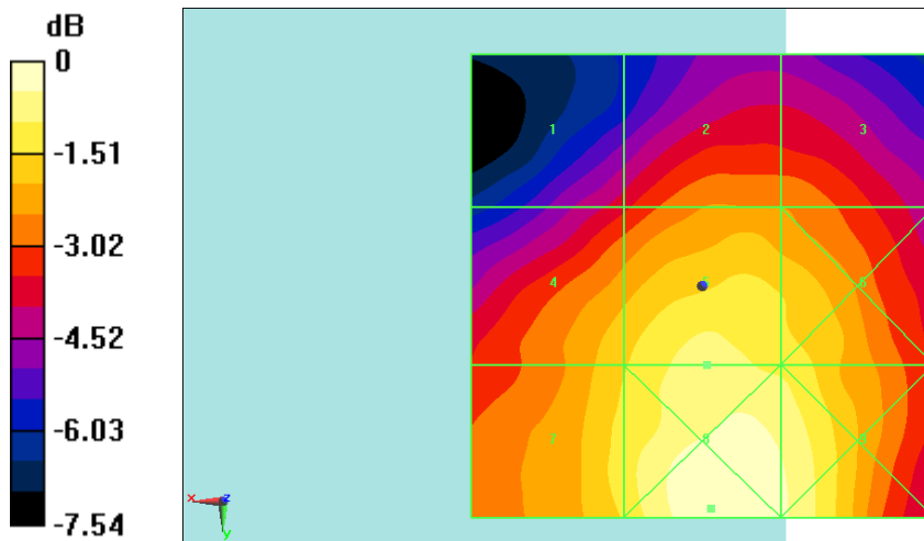
Fig B.5 HAC RF E-Field WiFi2.4G 11b
