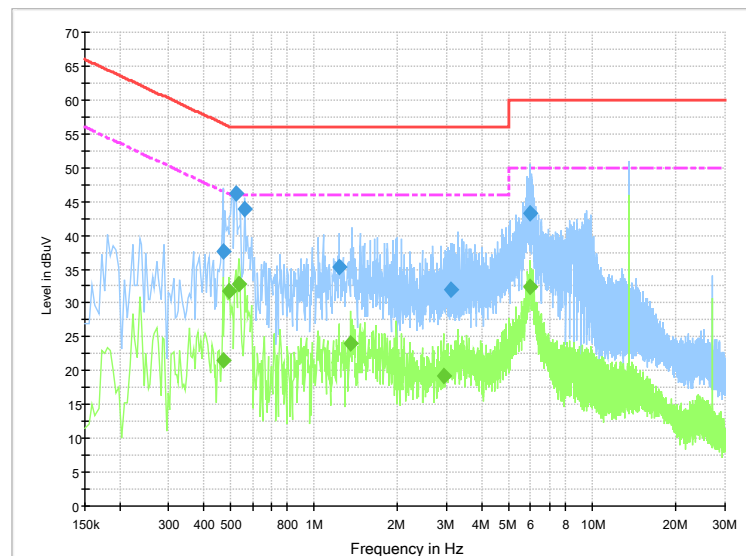
Figure B-11: Measurement results for Conducted Emission(NFC01-2)
