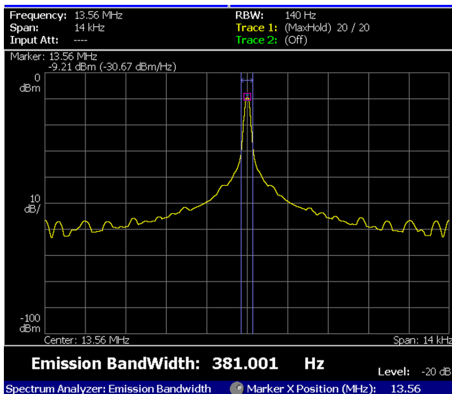
Figure B-9: Measurement results for 20dB Bandwidth
