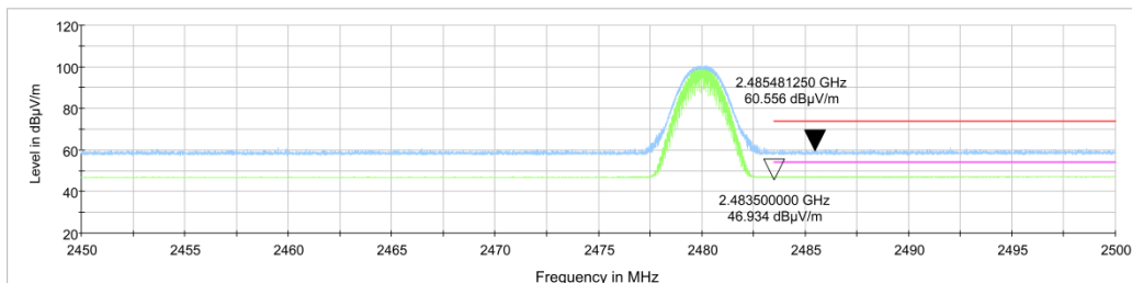
Fig.14. Frequency Band Edges: GFSK, Channel 78, Hopping Off, ch11, 2.45 GHz - 2.50GHz
