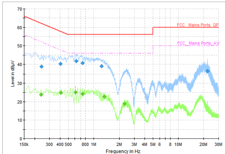
Fig.105 AC Power line Conducted Emission (Traffic), LE Coded
