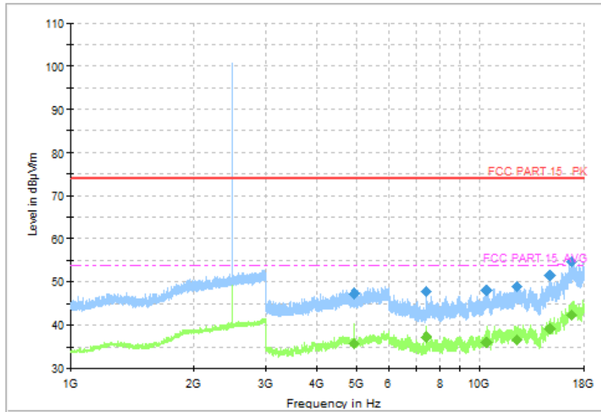
Fig.95 Radiated Spurious Emission (GFSK, Ch39, 1 GHz ~18 GHz), LE Coded S=2
