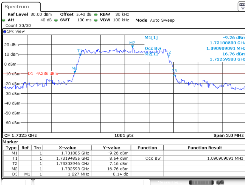
Band4-1.4MHz-QPSK-20175-6RB#0-1.091
