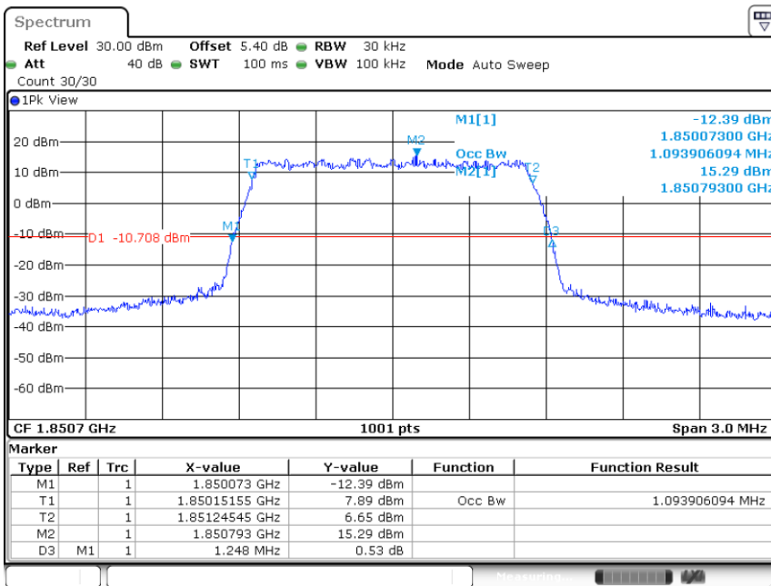
Band2-1.4MHz-QPSK-18607-6RB#0-1.094
