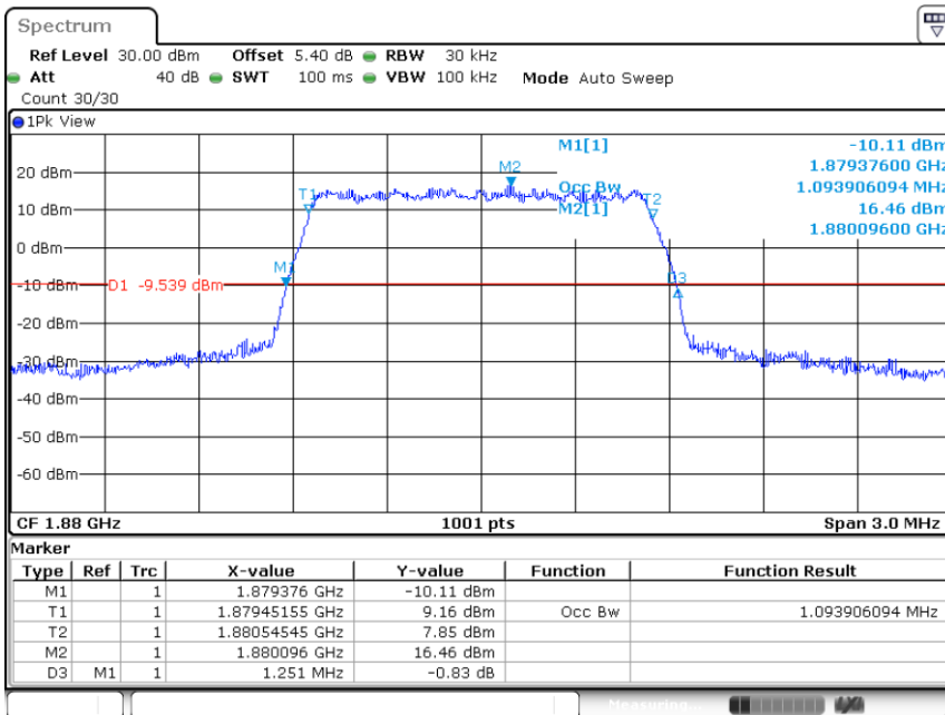
Band2-1.4MHz-QPSK-18900-6RB#0-1.094
