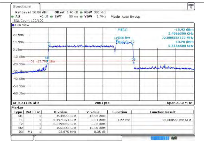
41-41-20MHz-5MHz-16QAM-16QAM-39750-39867-100RB#0-25RB#0
