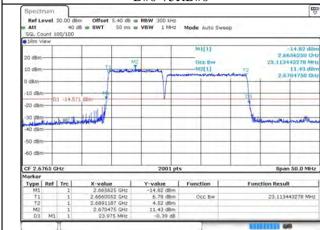
41-41-10MHz-15MHz-QPSK-QPSK-41395-41515-50R B#0-75RB#0
