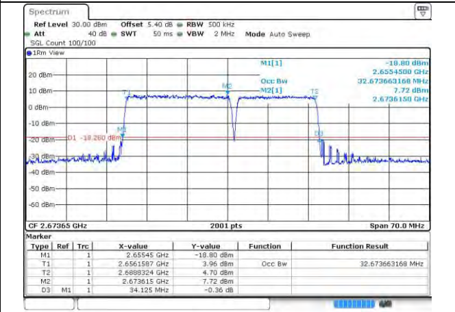
41-41-20MHz-15MHz-16QAM-16QAM-41341-41512-100RB#0-75RB#0
