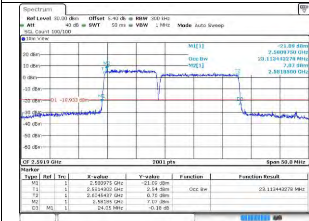
41-41-10MHz-15MHz-256QAM-256QAM-40549-40669-50RB#0-75RB#0
