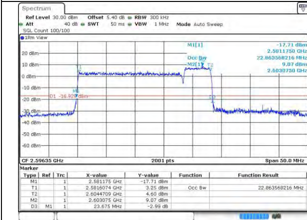
41-41-20MHz-5MHz-256QAM-256QAM-40595-40712-100RB#0-25RB#0
