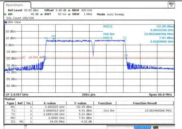
41-41-15MHz-10MHz-16QAM-16QAM-41417-41537-75RB#0-50RB#0
