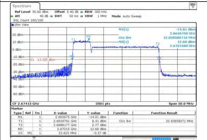
41-41-5MHz-20MHz-16QAM-16QAM-41373-41490-2 5RB#0-100RB#0
