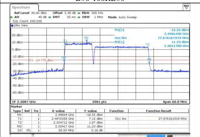
41-41-10MHz-20MHz-16QAM-16QAM-39705-39849-50RB#0-100RB#0
