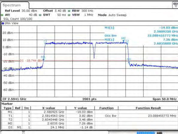
41-41-15MHz-10MHz-16QAM-16QAM-40571-40691-75RB#0-50RB#0
