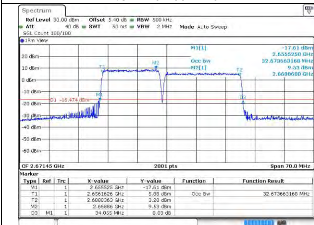
41-41-15MHz-20MHz-64QAM-64QAM-41319-41490-75RB#0-100RB#0
