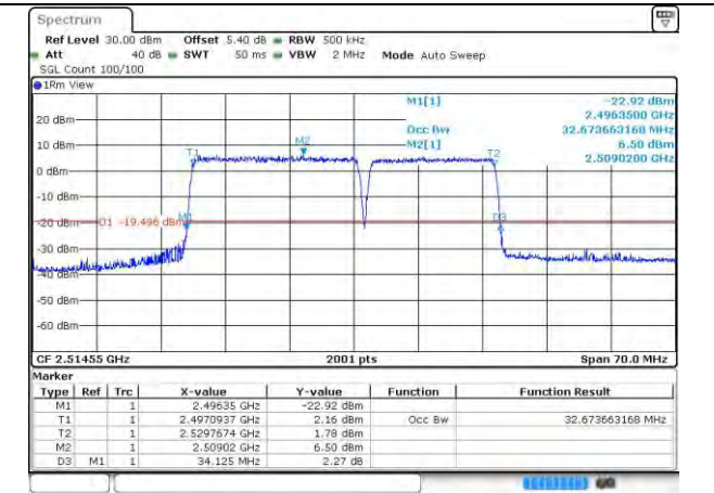
41-41-20MHz-15MHz-256QAM-256QAM-39750-39921-100RB#0-75RB#0
