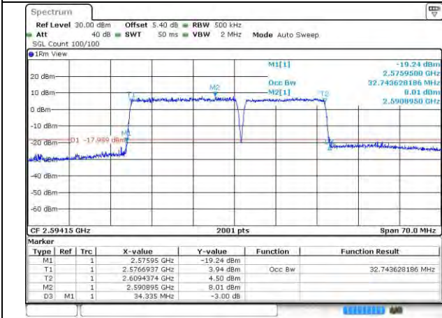
41-41-20MHz-15MHz-16QAM-16QAM-40546-40717-100RB#0-75RB#0
