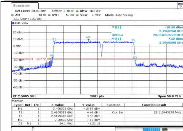
41-41-15MHz-10MHz-64QAM-64QAM-39725-39845-75RB#0-50RB#0
