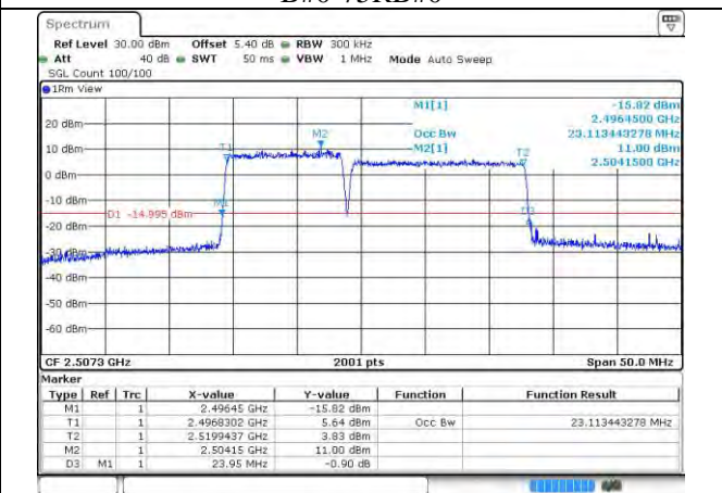
41-41-10MHz-15MHz-16QAM-16QAM-39703-39823-50RB#0-75RB#0
