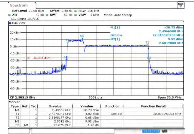
41-41-5MHz-20MHz-256QAM-256QAM-39683-39800 -25RB#0-100RB#0
