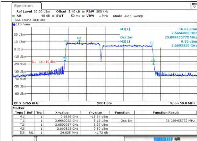
41-41-10MHz-15MHz-64QAM-64QAM-41395-41515-50RB#0-75RB#0
