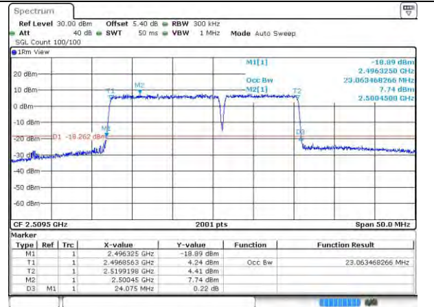
41-41-15MHz-10MHz-16QAM-16QAM-39725-39845-75RB#0-50RB#0
