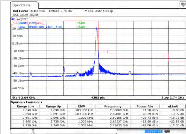
CA_41C_100RB+100RB_QPSK_41292+41490_OR B#0+1RB#99
