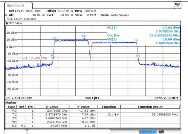
41-41-15MHz-20MHz-QPSK-QPSK-40523-40694-75R B#0-100RB#0
