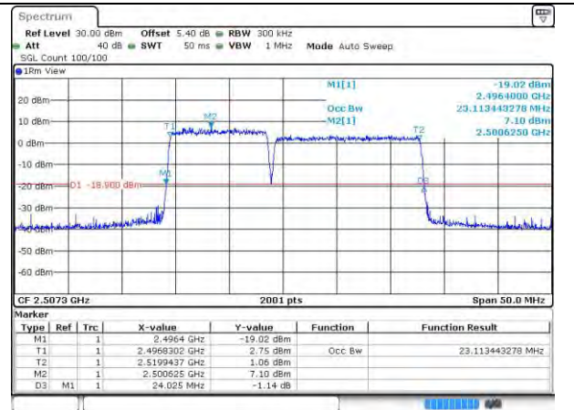
41-41-10MHz-15MHz-256QAM-256QAM-39703-39823-50RB#0-75RB#0
