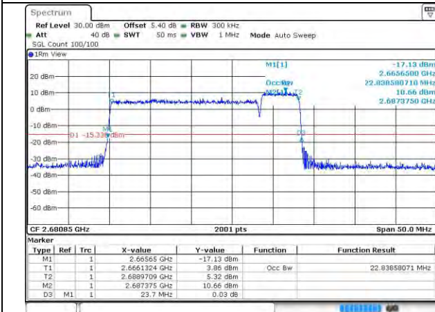
41-41-20MHz-5MHz-64QAM-64QAM-41440-41557-1 OORB#0-25RB#0
