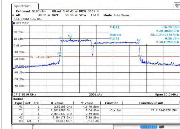
41-41-10MHz-15MHz-16QAM-16QAM-40549-40669-50RB#0-75RB#0
