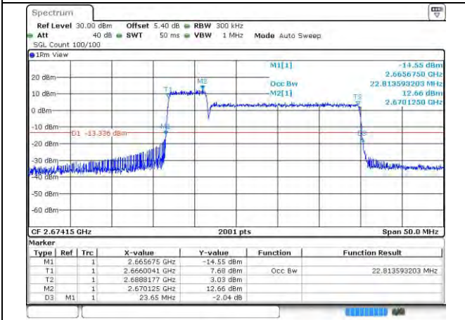
41-41-5MHz-20MHz-64QAM-64QAM-41373-41490-2 5RB#0-100RB#0
