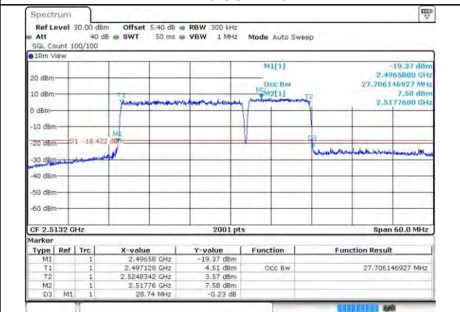
41-41-20MHz-10MHz-16QAM-16QAM-39750-39894- 100RB#0-50RB#0
