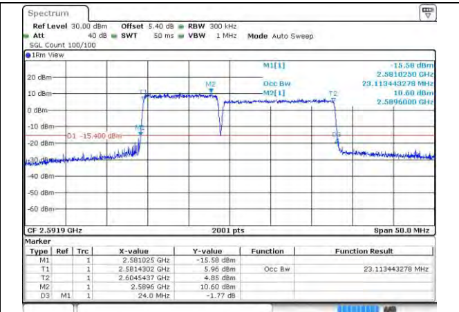
41-41-10MHz-15MHz-QPSK-QPSK-40549-40669-50R B#0-75RB#0
