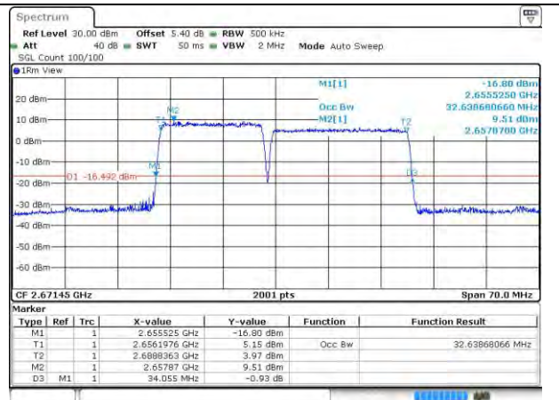
41-41-15MHz-20MHz-16QAM-16QAM-41319-41490-75RB#0-100RB#0
