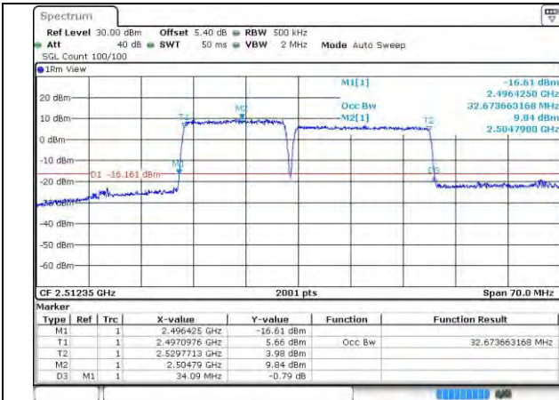
41-41-15MHz-20MHz-QPSK-QPSK-39728-39899-75R B#0-100RB#0
