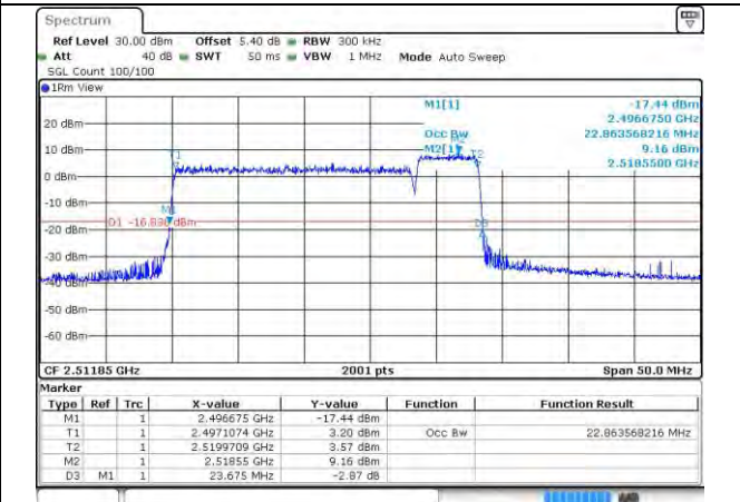
41-41-20MHz-5MHz-256QAM-256QAM-39750-39867-100RB#0-25RB#0
