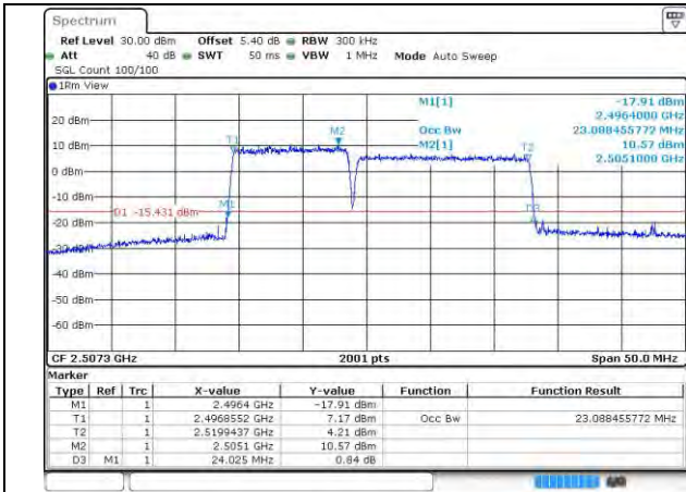
41-41-10MHz-15MHz-QPSK-QPSK-39703-39823-50R B#0-75RB#0
