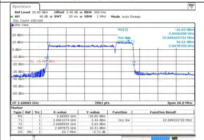
41-41-20MHz-5MHz-16QAM-16QAM-41440-41557-100RB#0-25RB#0
