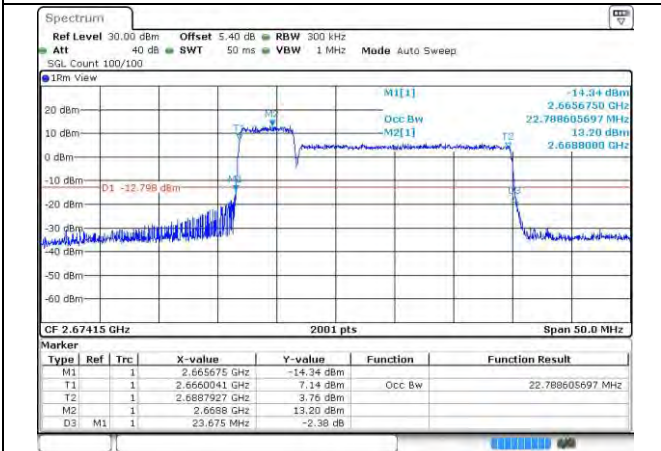
41-41-5MHz-20MHz-QPSK-QPSK-41373-41490-25R B#0-100RB#0
