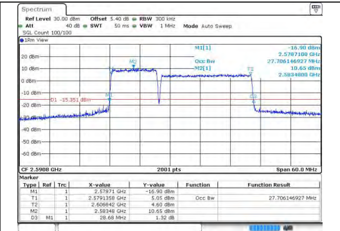
41-41-10MHz-20MHz-QPSK-QPSK-40526-40670-50R B#0-100RB#0
