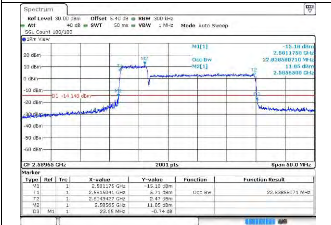
41-41-5MHz-20MHz-16QAM-16QAM-40528-40645-2 5RB#0-100RB#0
