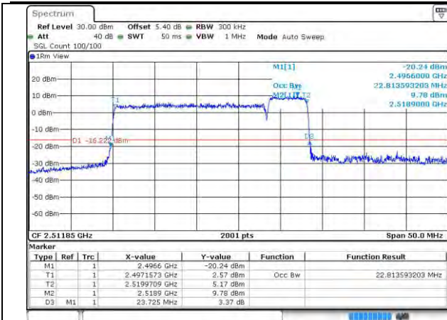
41-41-20MHz-5MHz-64QAM-64QAM-39750-39867-1 OORB#0-25RB#0
