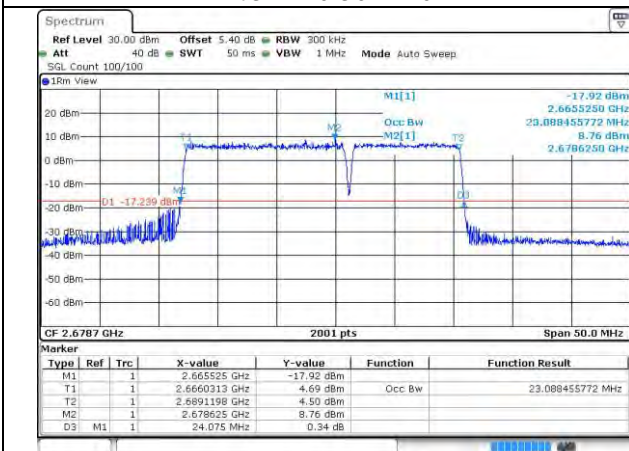
41-41-15MHz-10MHz-64QAM-64QAM-41417-41537-75RB#0-50RB#0
