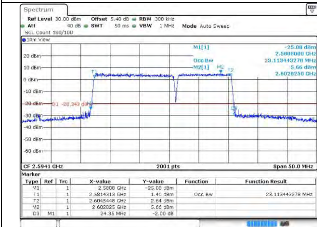
41-41-15MHz-10MHz-256QAM-256QAM-40571-40691-7-75RB#0-50RB#0
