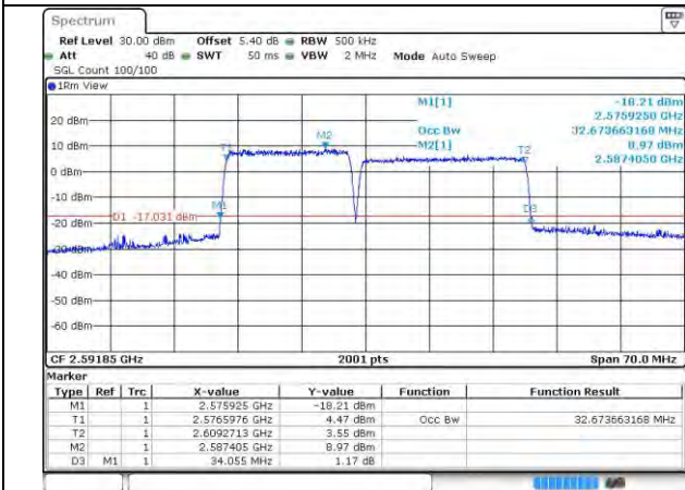
41-41-15MHz-20MHz-16QAM-16QAM-40523-40694-75RB#0-100RB#0
