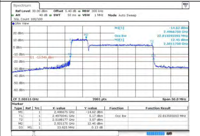
41-41-5MHz-20MHz-16QAM-16QAM-39683-39800-2 5RB#0-100RB#0
