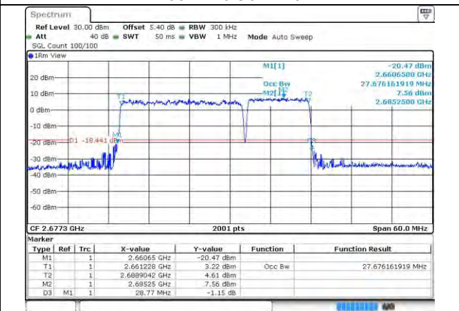
41-41-20MHz-10MHz-16QAM-16QAM-41391-41535- 100RB#0-50RB#0
