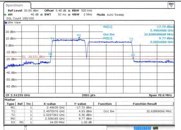
41-41-15MHz-20MHz-16QAM-16QAM-39728-39899-75RB#0-100RB#0
