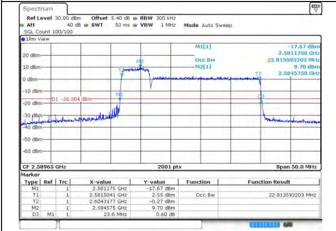
41-41-5MHz-20MHz-256QAM-256QAM-40528-40645 -25RB#0-100RB#0
