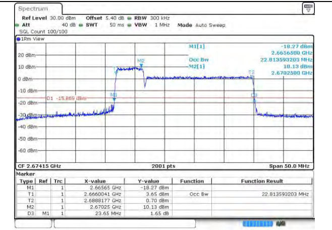
41-41-5MHz-20MHz-256QAM-256QAM-41373-41490 -25RB#0-100RB#0
