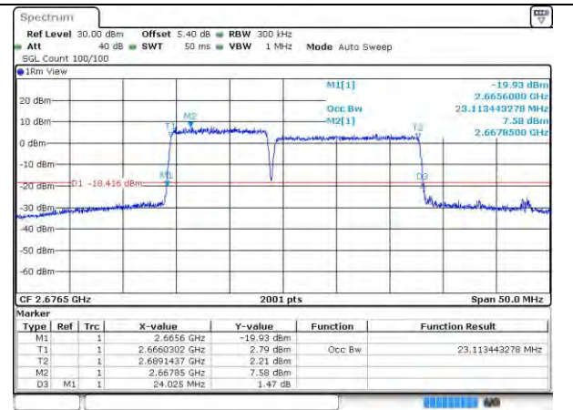
41-41-10MHz-15MHz-256QAM-256QAM-41395-41515-50RB#0-75RB#0
