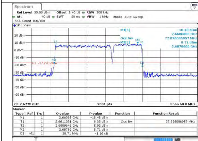
41-41-20MHz-10MHz-QPSK-QPSK-41391-41535-100 RB#0-50RB#0
