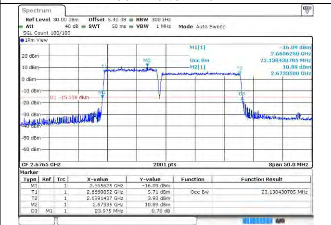
41-41-10MHz-15MHz-16QAM-16QAM-41395-41515-50RB#0-75RB#0
