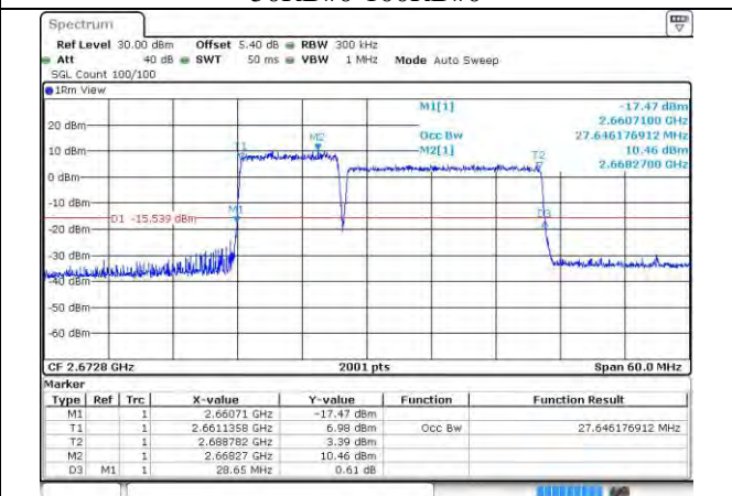
41-41-10MHz-20MHz-16QAM-16QAM-41346-41490-50RB#0-100RB#0
