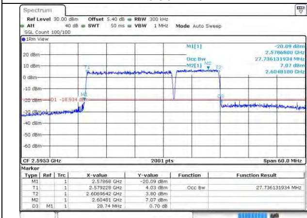
41-41-20MHz-10MHz-16QAM-16QAM-40571-40715- 100RB#0-50RB#0
