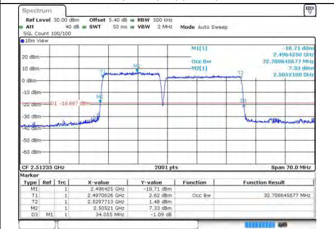
41-41-15MHz-20MHz-256QAM-256QAM-39728-3989-9-75RB#0-100RB#0
