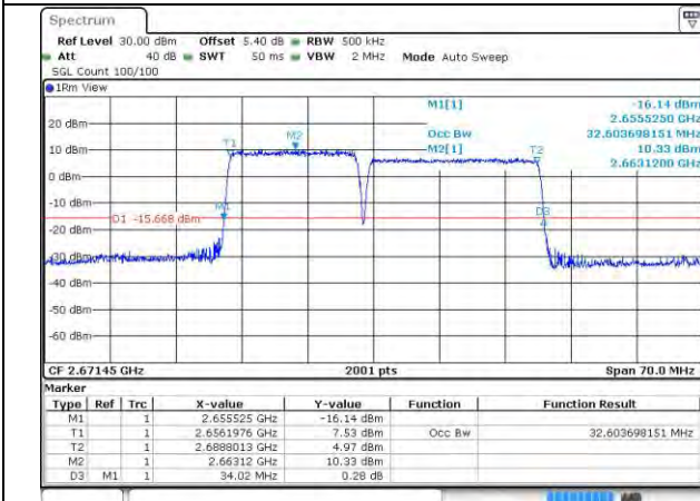
41-41-15MHz-20MHz-QPSK-QPSK-41319-41490-75R B#0-100RB#0
